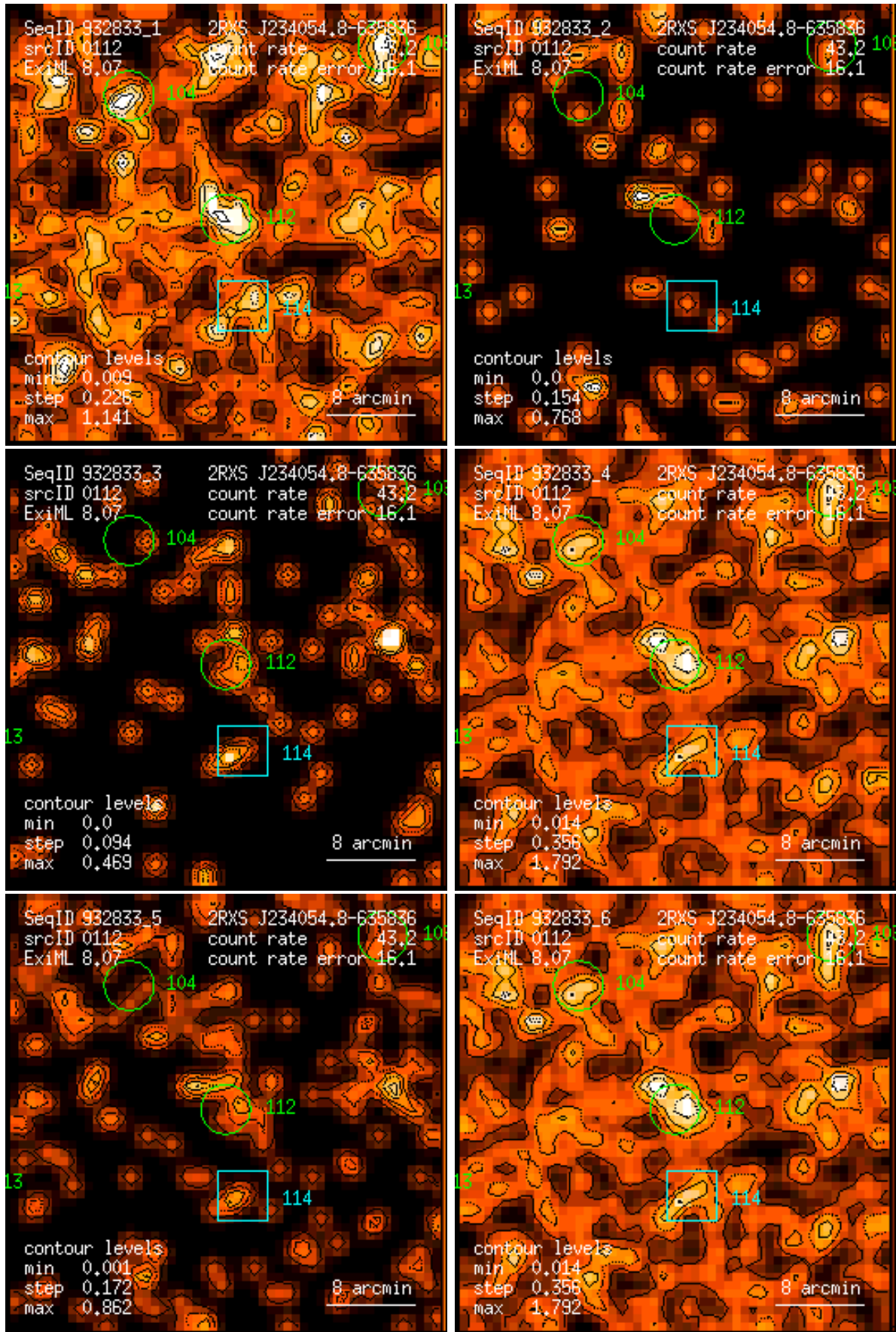
Figure 112: RASS 932833: detection 0112: band rate images, Gaussian filter: (1) PSPC channels 11 – 41, (2) 52 – 90, (3) 91 – 201, (4) 11 – 235, (5) 52 – 201, (6) 11 – 201. Broad band rates in counts/ks. Band rate contour levels in counts/ks/arcmin 2 .
