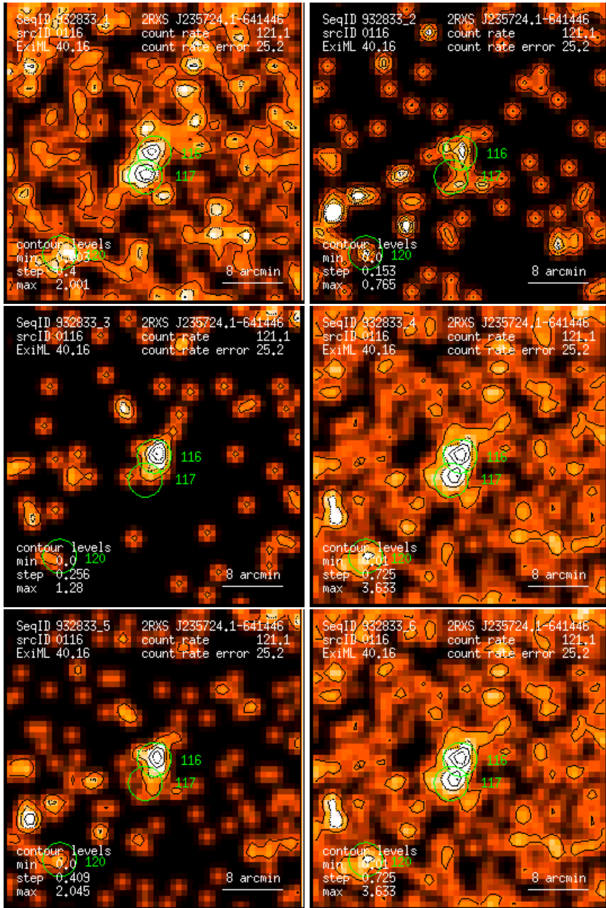
Figure 116: RASS 932833: detection 0116: band rate images, Gaussian filter: (1) PSPC channels 11 – 41, (2) 52 – 90, (3) 91 – 201, (4) 11 – 235, (5) 52 – 201, (6) 11 – 201. Broad band rates in counts/ks. Band rate contour levels in counts/ks/arcmin 2 .
