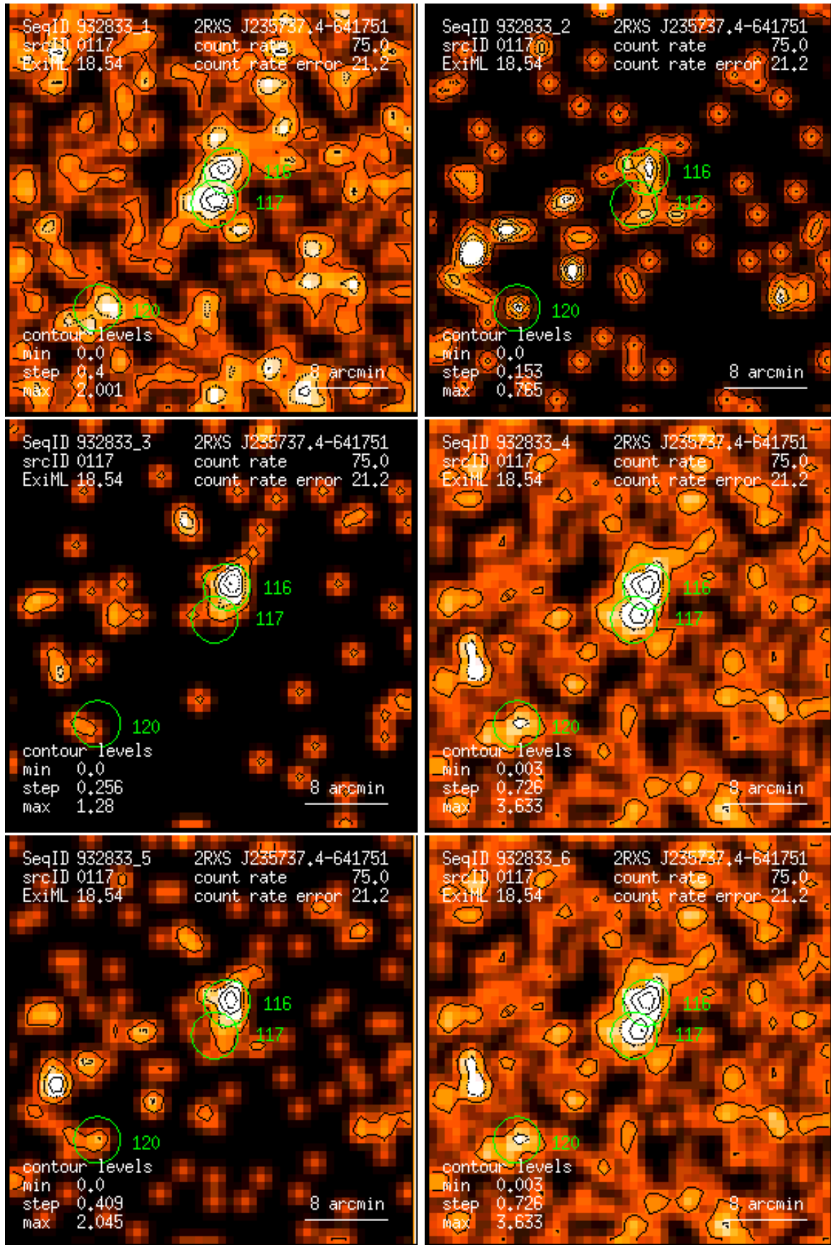
Figure 117: RASS 932833: detection 0117: band rate images, Gaussian filter: (1) PSPC channels 11 – 41, (2) 52 – 90, (3) 91 – 201, (4) 11 – 235, (5) 52 – 201, (6) 11 – 201. Broad band rates in counts/ks. Band rate contour levels in counts/ks/arcmin 2 .
