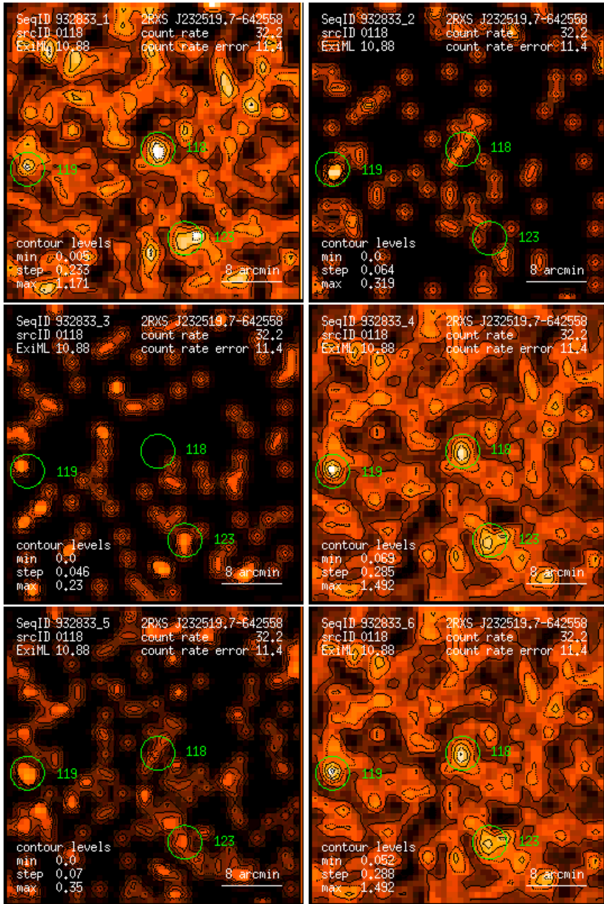
Figure 118: RASS 932833: detection 0118: band rate images, Gaussian filter: (1) PSPC channels 11 – 41, (2) 52 – 90, (3) 91 – 201, (4) 11 – 235, (5) 52 – 201, (6) 11 – 201. Broad band rates in counts/ks. Band rate contour levels in counts/ks/arcmin 2 .
