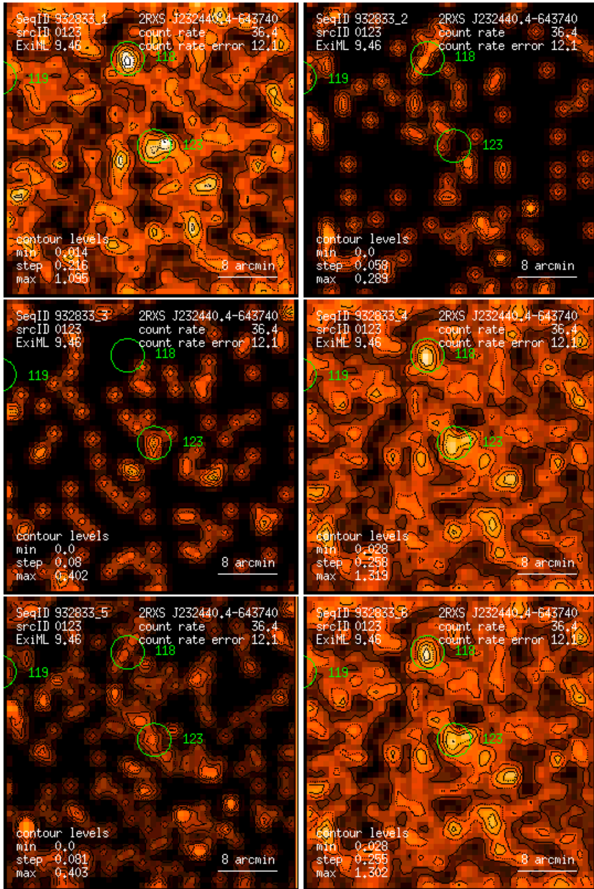
Figure 123: RASS 932833: detection 0123: band rate images, Gaussian filter: (1) PSPC channels 11 – 41, (2) 52 – 90, (3) 91 – 201, (4) 11 – 235, (5) 52 – 201, (6) 11 – 201. Broad band rates in counts/ks. Band rate contour levels in counts/ks/arcmin 2 .
