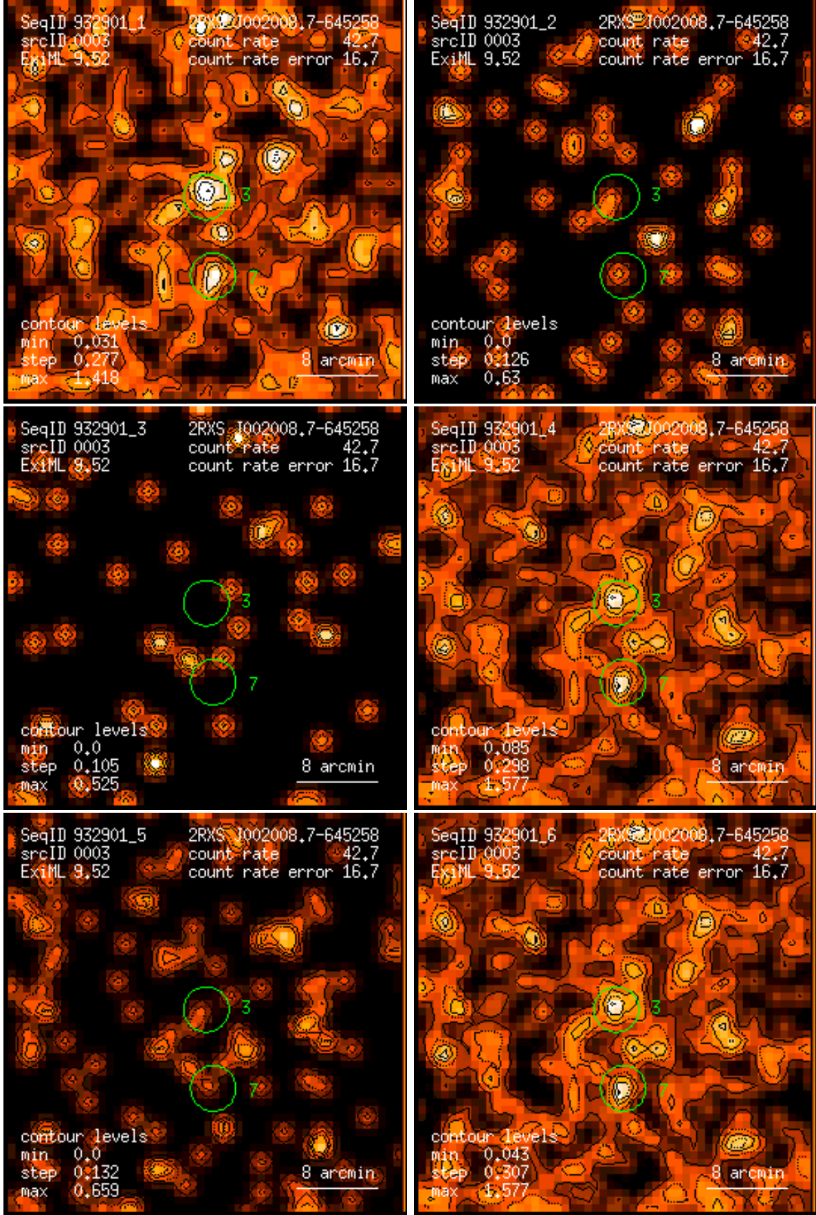
Figure 3: RASS 932901: detection 0003: band rate images, Gaussian filter: (1) PSPC channels 11 – 41, (2) 52 – 90, (3) 91 – 201, (4) 11 – 235, (5) 52 – 201, (6) 11 – 201. Broad band rates in counts/ks. Band rate contour levels in counts/ks/arcmin 2 .
