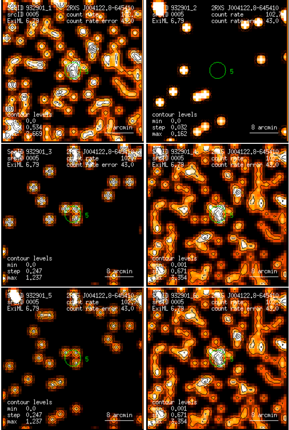
Figure 5: RASS 932901: detection 0005: band rate images, Gaussian filter: (1) PSPC channels 11 – 41, (2) 52 – 90, (3) 91 – 201, (4) 11 – 235, (5) 52 – 201, (6) 11 – 201. Broad band rates in counts/ks. Band rate contour levels in counts/ks/arcmin 2 .
