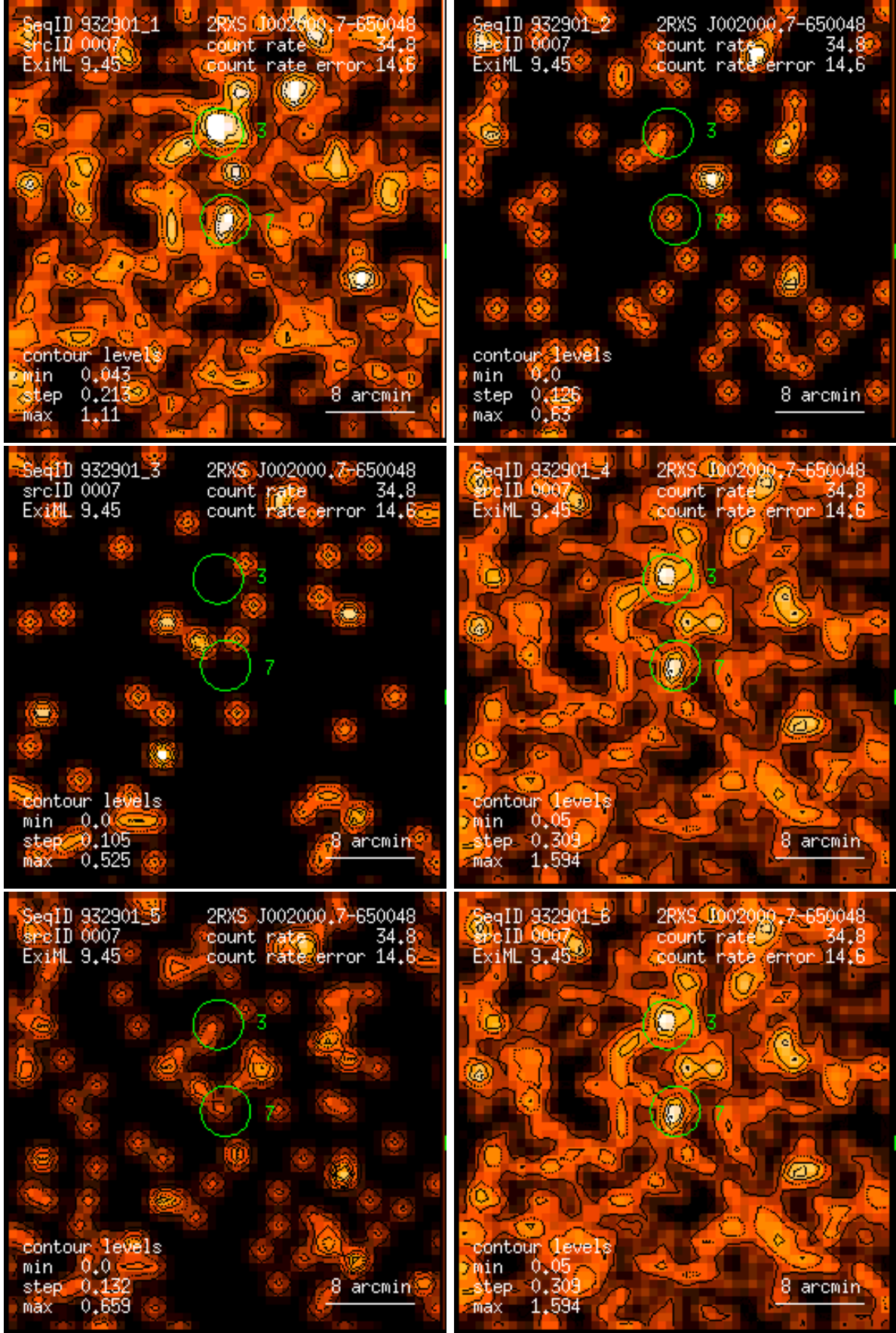
Figure 7: RASS 932901: detection 0007: band rate images, Gaussian filter: (1) PSPC channels 11 – 41, (2) 52 – 90, (3) 91 – 201, (4) 11 – 235, (5) 52 – 201, (6) 11 – 201. Broad band rates in counts/ks. Band rate contour levels in counts/ks/arcmin 2 .
