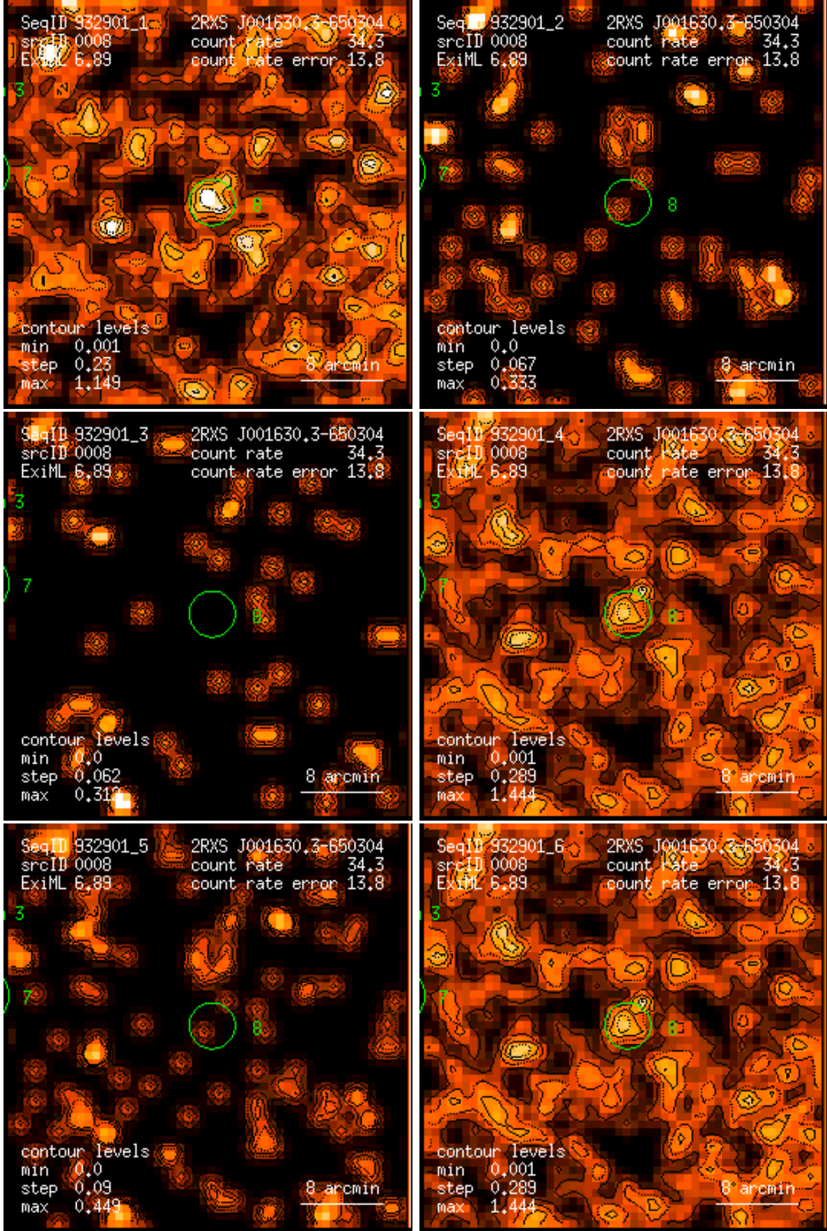
Figure 8: RASS 932901: detection 0008: band rate images, Gaussian filter: (1) PSPC channels 11 – 41, (2) 52 – 90, (3) 91 – 201, (4) 11 – 235, (5) 52 – 201, (6) 11 – 201. Broad band rates in counts/ks. Band rate contour levels in counts/ks/arcmin 2 .
