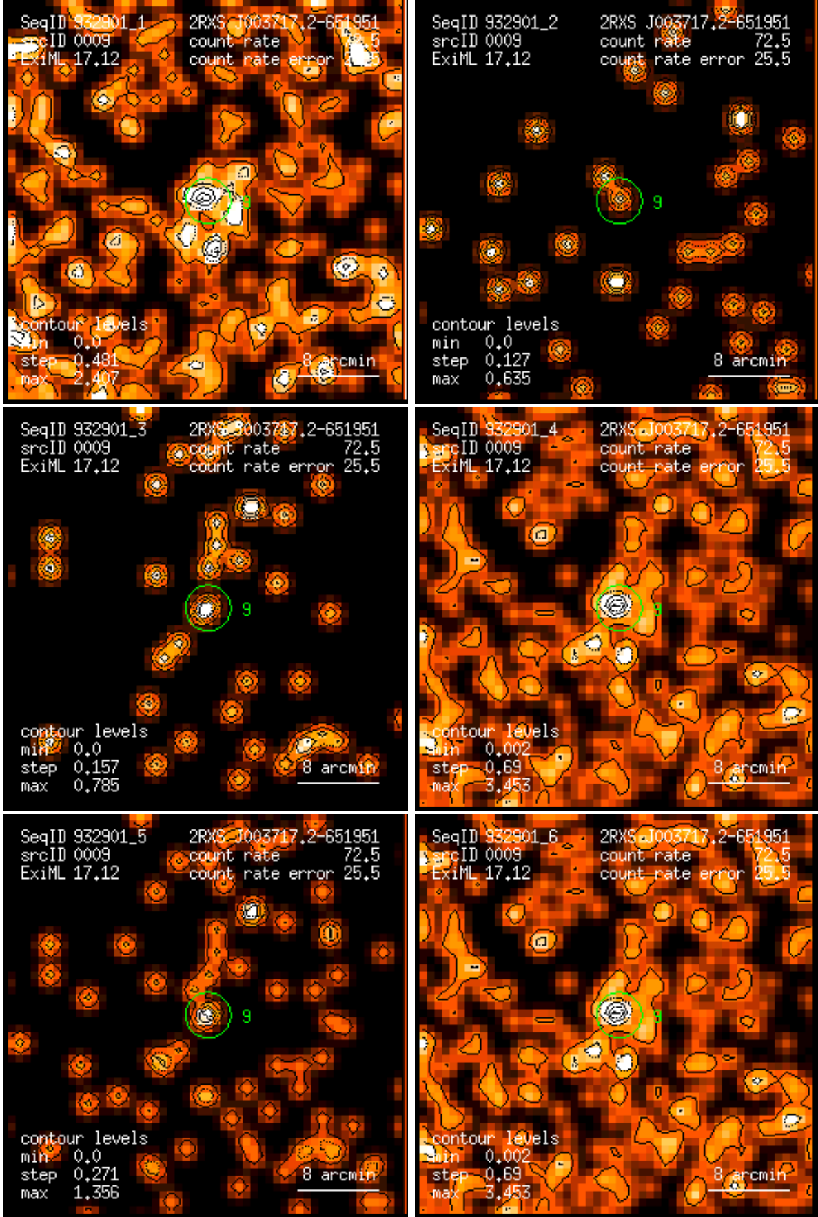
Figure 9: RASS 932901: detection 0009: band rate images, Gaussian filter: (1) PSPC channels 11 – 41, (2) 52 – 90, (3) 91 – 201, (4) 11 – 235, (5) 52 – 201, (6) 11 – 201. Broad band rates in counts/ks. Band rate contour levels in counts/ks/arcmin 2 .
