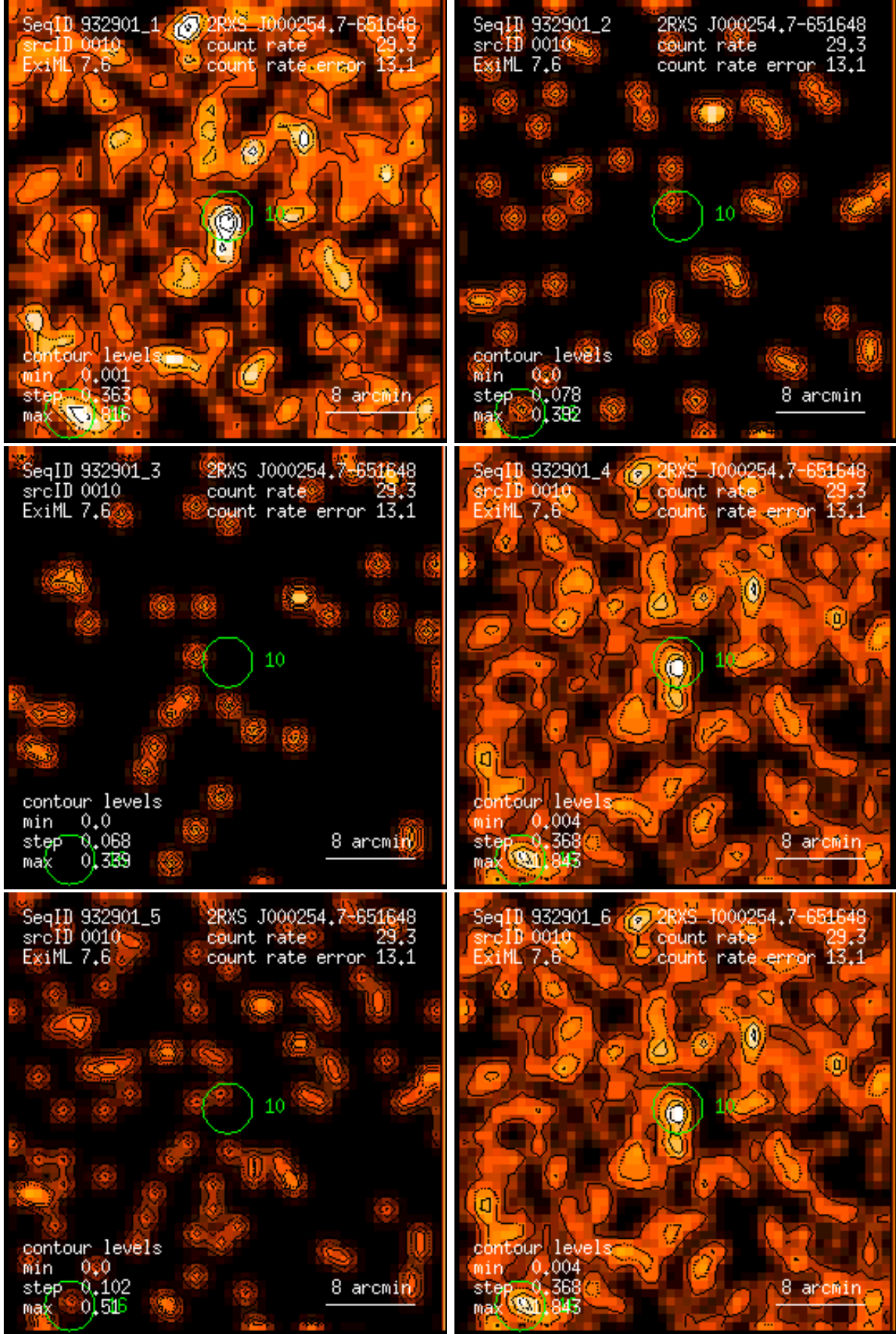
Figure 10: RASS 932901: detection 0010: band rate images, Gaussian filter: (1) PSPC channels 11 – 41, (2) 52 – 90, (3) 91 – 201, (4) 11 – 235, (5) 52 – 201, (6) 11 – 201. Broad band rates in counts/ks. Band rate contour levels in counts/ks/arcmin 2 .
