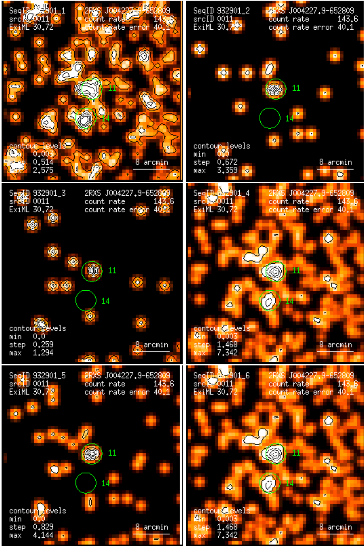
Figure 11: RASS 932901: detection 0011: band rate images, Gaussian filter: (1) PSPC channels 11 – 41, (2) 52 – 90, (3) 91 – 201, (4) 11 – 235, (5) 52 – 201, (6) 11 – 201. Broad band rates in counts/ks. Band rate contour levels in counts/ks/arcmin 2 .
