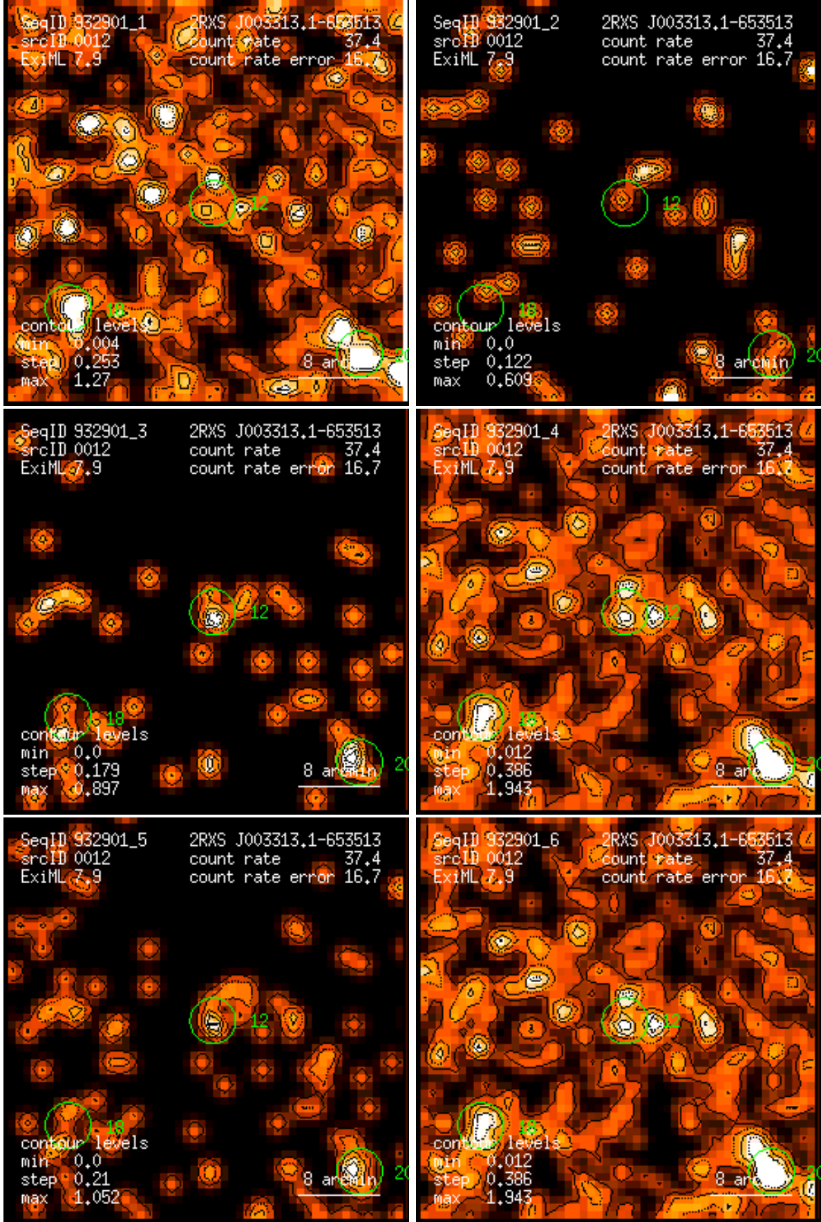
Figure 12: RASS 932901: detection 0012: band rate images, Gaussian filter: (1) PSPC channels 11 – 41, (2) 52 – 90, (3) 91 – 201, (4) 11 – 235, (5) 52 – 201, (6) 11 – 201. Broad band rates in counts/ks. Band rate contour levels in counts/ks/arcmin 2 .
