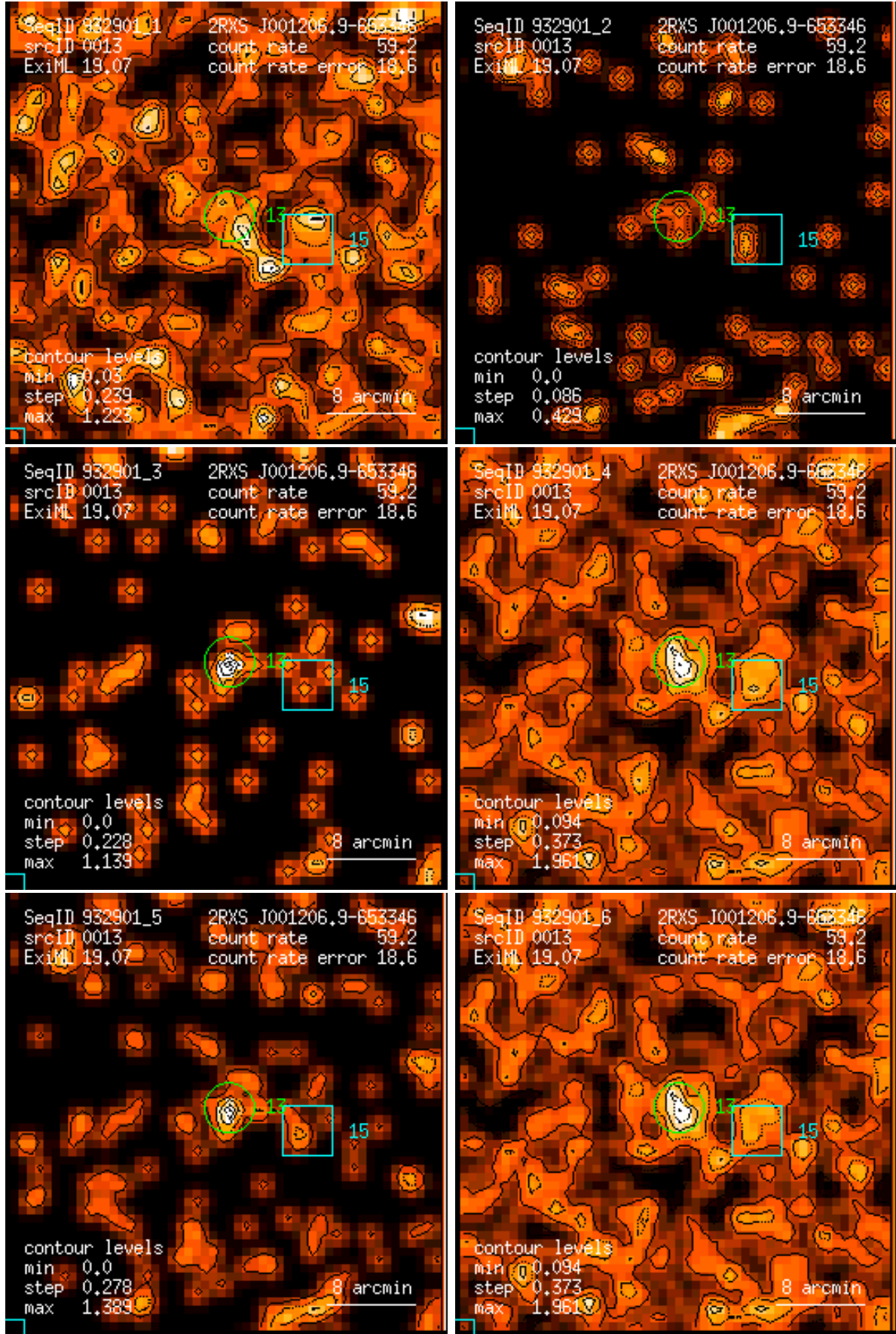
Figure 13: RASS 932901: detection 0013: band rate images, Gaussian filter: (1) PSPC channels 11 – 41, (2) 52 – 90, (3) 91 – 201, (4) 11 – 235, (5) 52 – 201, (6) 11 – 201. Broad band rates in counts/ks. Band rate contour levels in counts/ks/arcmin 2 .
