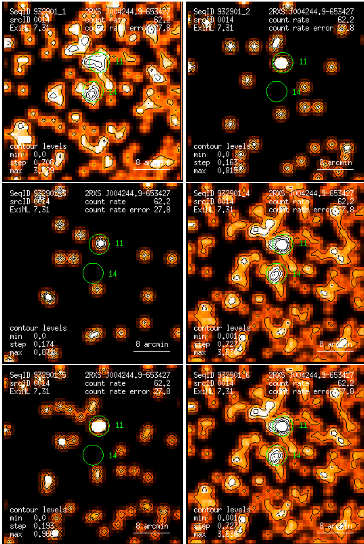
Figure 14: RASS 932901: detection 0014: band rate images, Gaussian filter: (1) PSPC channels 11 – 41, (2) 52 – 90, (3) 91 – 201, (4) 11 – 235, (5) 52 – 201, (6) 11 – 201. Broad band rates in counts/ks. Band rate contour levels in counts/ks/arcmin 2 .
