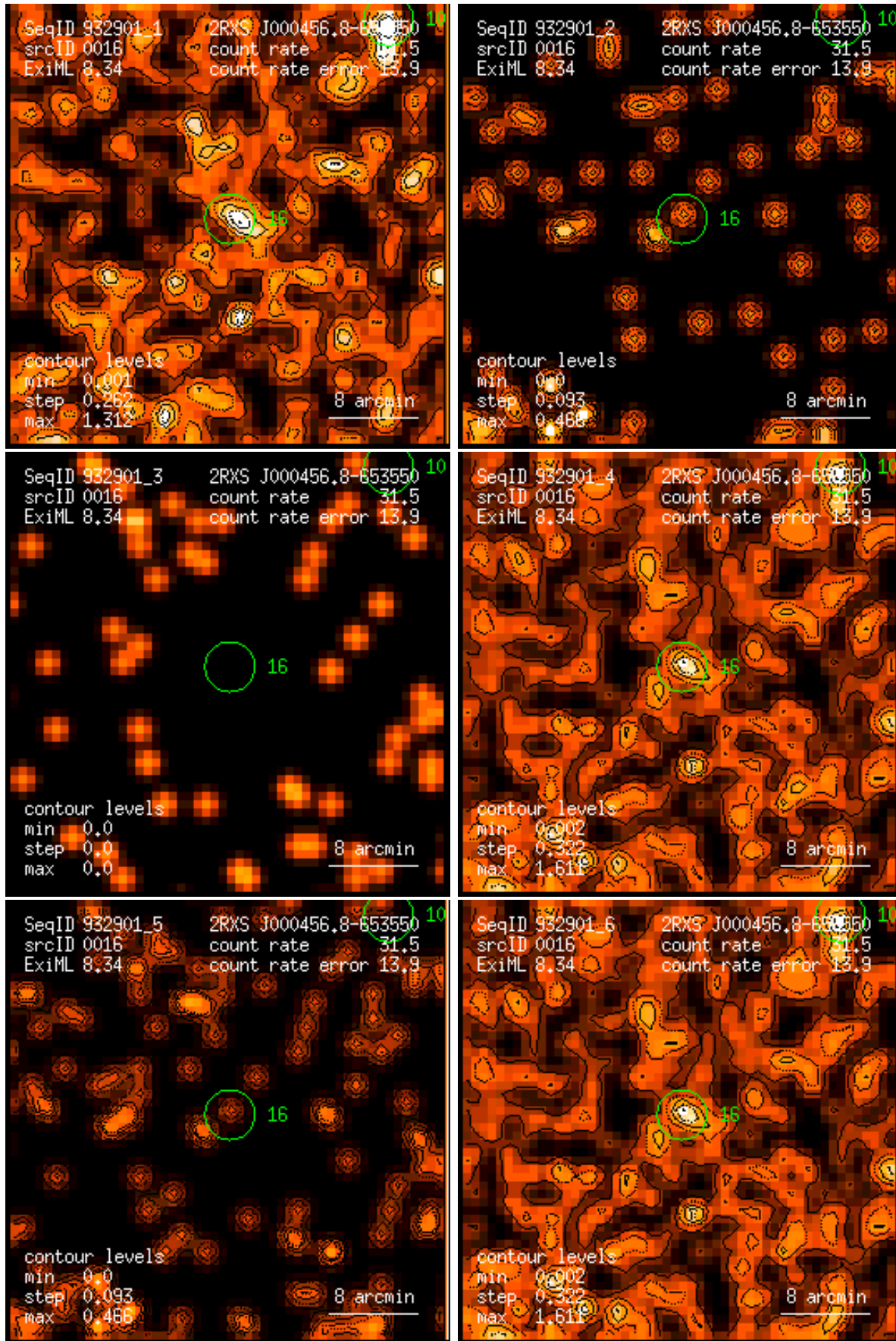
Figure 16: RASS 932901: detection 0016: band rate images, Gaussian filter: (1) PSPC channels 11 – 41, (2) 52 – 90, (3) 91 – 201, (4) 11 – 235, (5) 52 – 201, (6) 11 – 201. Broad band rates in counts/ks. Band rate contour levels in counts/ks/arcmin 2 .
