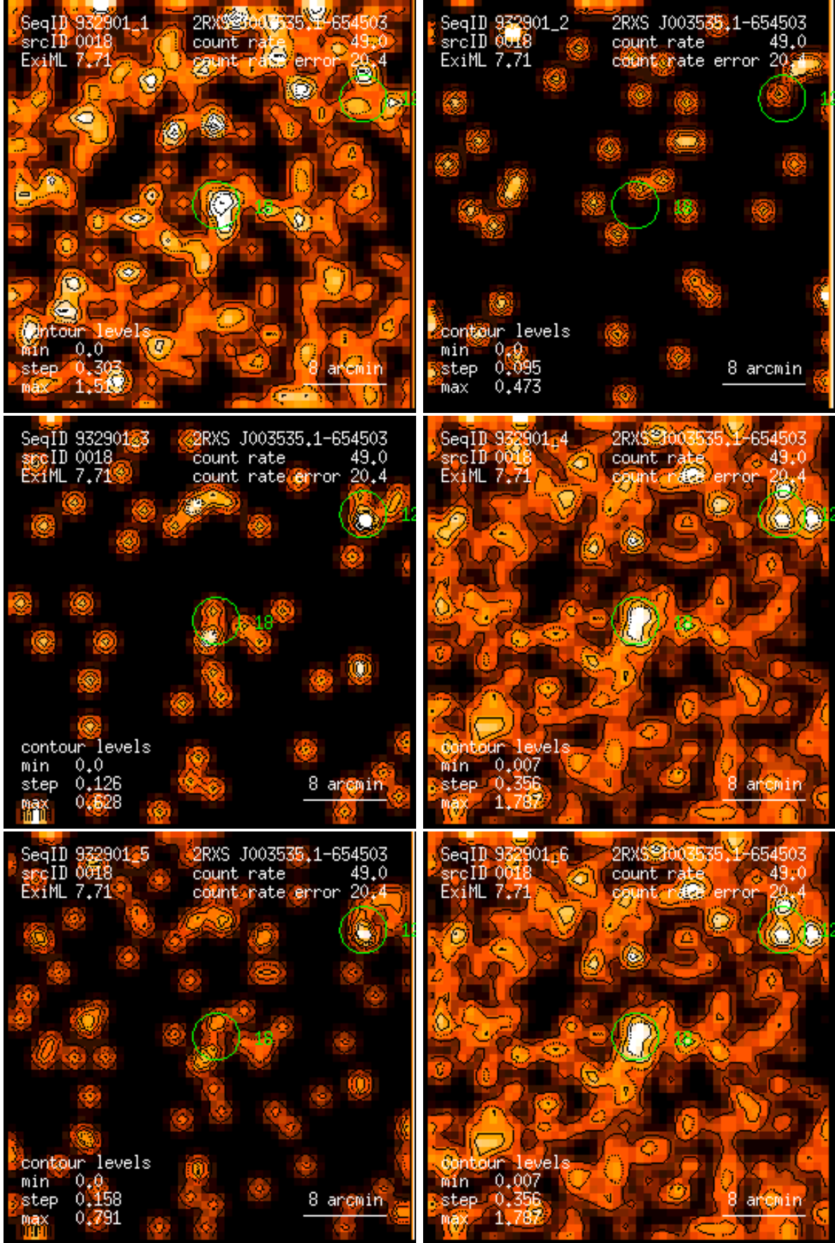
Figure 18: RASS 932901: detection 0018: band rate images, Gaussian filter: (1) PSPC channels 11 – 41, (2) 52 – 90, (3) 91 – 201, (4) 11 – 235, (5) 52 – 201, (6) 11 – 201. Broad band rates in counts/ks. Band rate contour levels in counts/ks/arcmin 2 .
