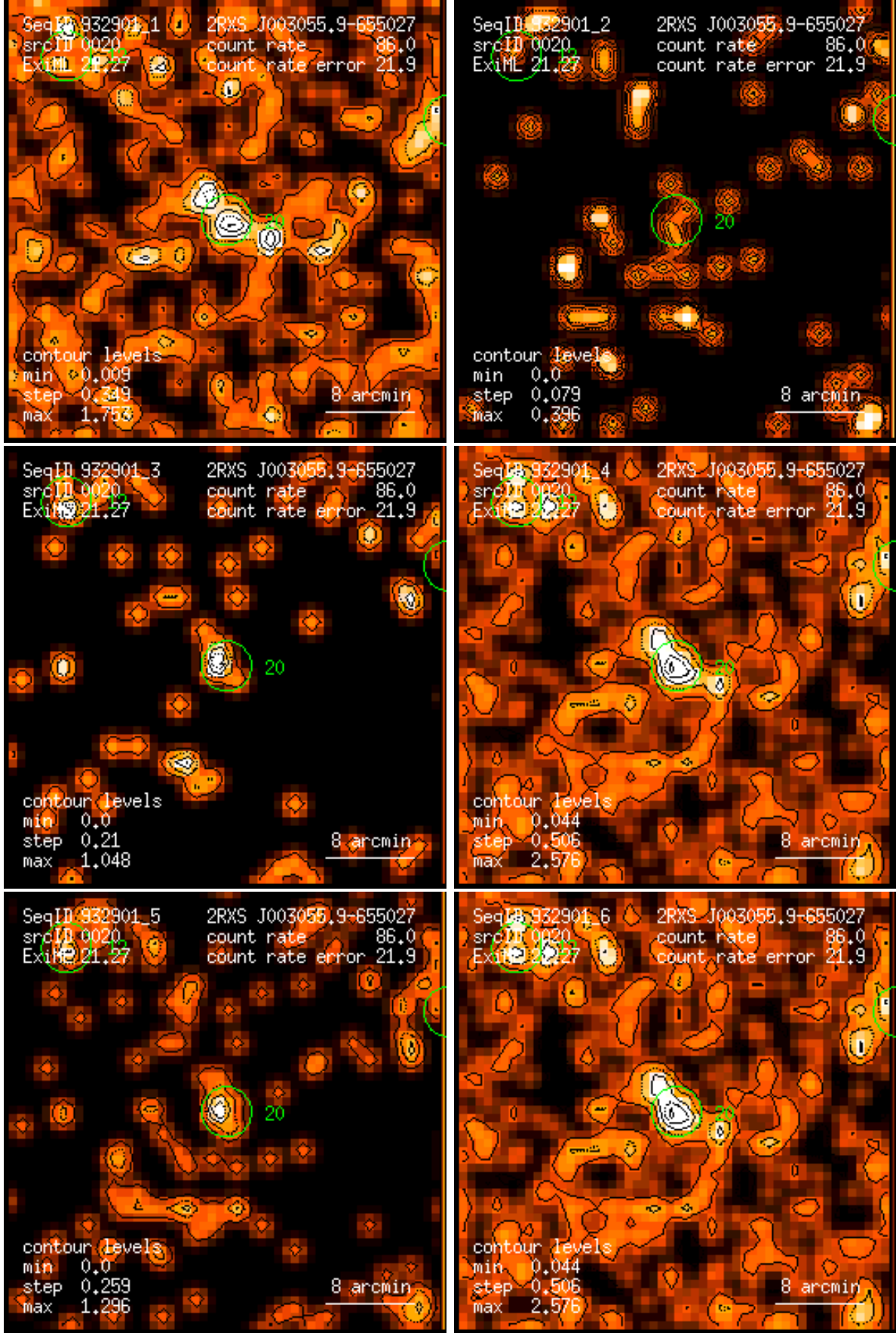
Figure 20: RASS 932901: detection 0020: band rate images, Gaussian filter: (1) PSPC channels 11 – 41, (2) 52 – 90, (3) 91 – 201, (4) 11 – 235, (5) 52 – 201, (6) 11 – 201. Broad band rates in counts/ks. Band rate contour levels in counts/ks/arcmin 2 .
