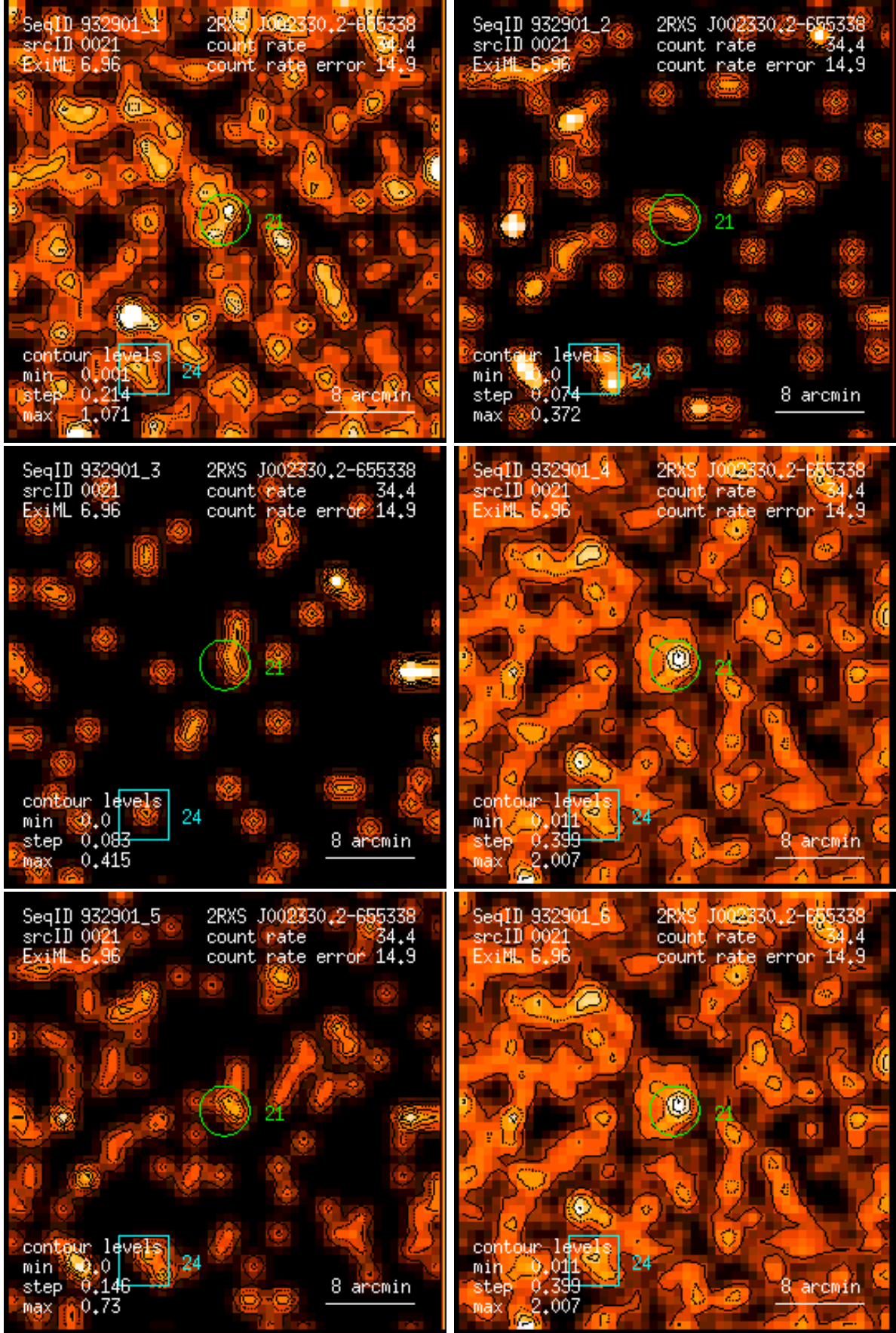
Figure 21: RASS 932901: detection 0021: band rate images, Gaussian filter: (1) PSPC channels 11 – 41, (2) 52 – 90, (3) 91 – 201, (4) 11 – 235, (5) 52 – 201, (6) 11 – 201. Broad band rates in counts/ks. Band rate contour levels in counts/ks/arcmin 2 .
