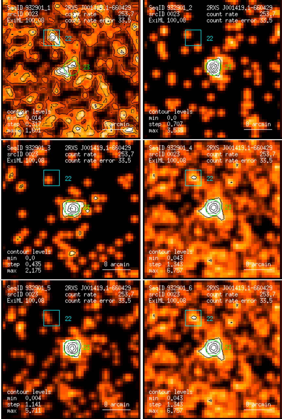
Figure 23: RASS 932901: detection 0023: band rate images, Gaussian filter: (1) PSPC channels 11 – 41, (2) 52 – 90, (3) 91 – 201, (4) 11 – 235, (5) 52 – 201, (6) 11 – 201. Broad band rates in counts/ks. Band rate contour levels in counts/ks/arcmin 2 .
