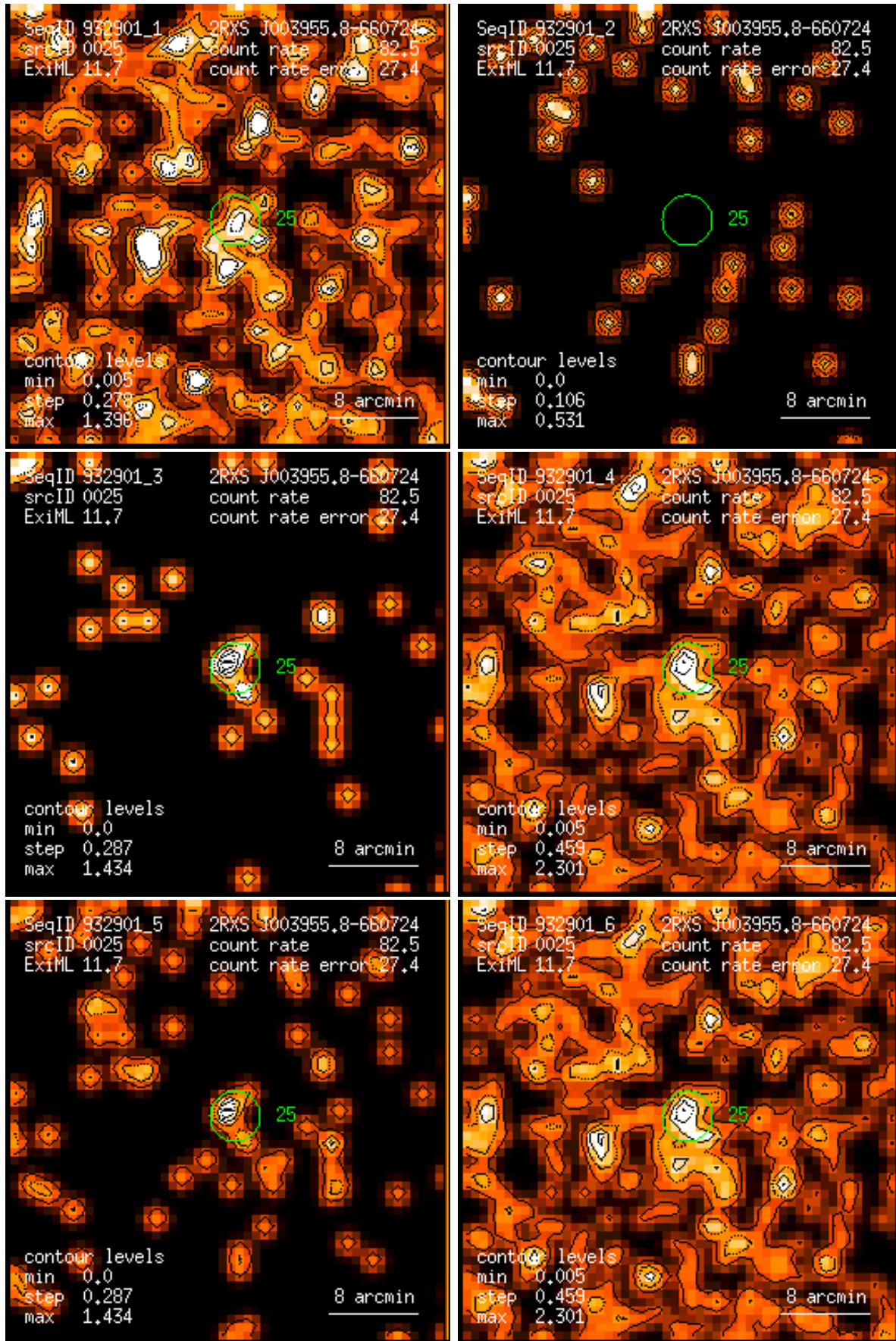
Figure 25: RASS 932901: detection 0025: band rate images, Gaussian filter: (1) PSPC channels 11 – 41, (2) 52 – 90, (3) 91 – 201, (4) 11 – 235, (5) 52 – 201, (6) 11 – 201. Broad band rates in counts/ks. Band rate contour levels in counts/ks/arcmin 2 .
