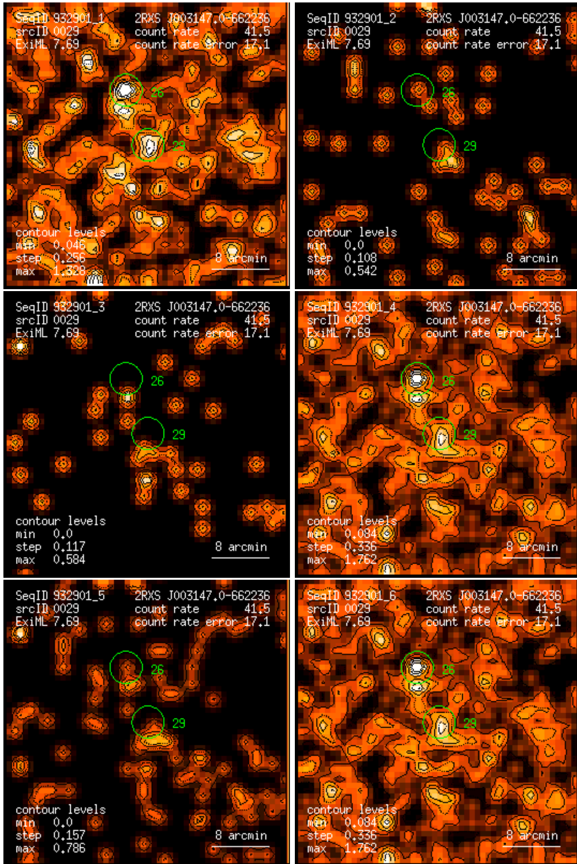
Figure 29: RASS 932901: detection 0029: band rate images, Gaussian filter: (1) PSPC channels 11 – 41, (2) 52 – 90, (3) 91 – 201, (4) 11 – 235, (5) 52 – 201, (6) 11 – 201. Broad band rates in counts/ks. Band rate contour levels in counts/ks/arcmin 2 .
