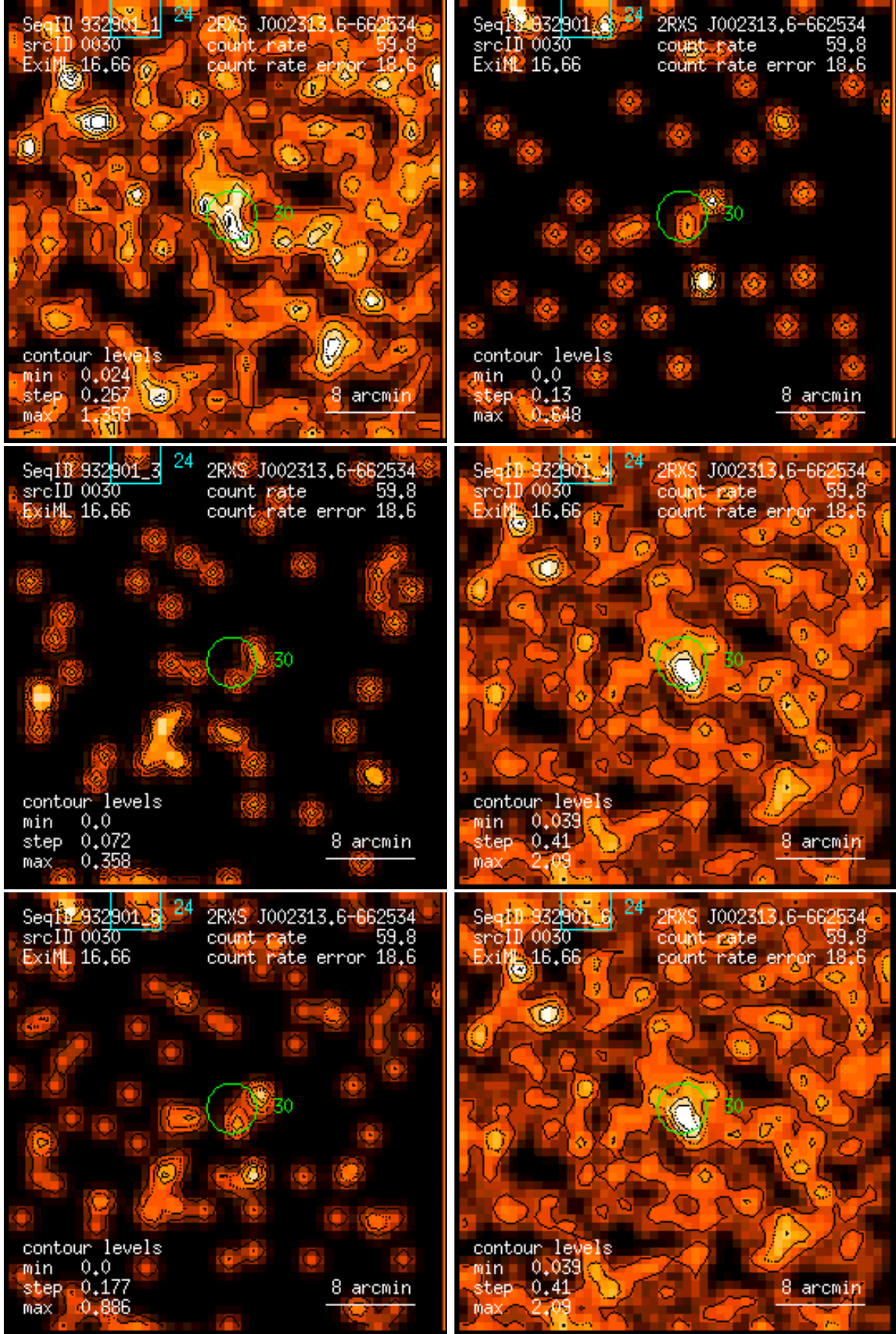
Figure 30: RASS 932901: detection 0030: band rate images, Gaussian filter: (1) PSPC channels 11 – 41, (2) 52 – 90, (3) 91 – 201, (4) 11 – 235, (5) 52 – 201, (6) 11 – 201. Broad band rates in counts/ks. Band rate contour levels in counts/ks/arcmin 2 .
