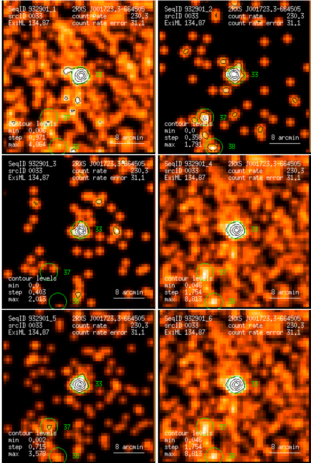
Figure 33: RASS 932901: detection 0033: band rate images, Gaussian filter: (1) PSPC channels 11 – 41, (2) 52 – 90, (3) 91 – 201, (4) 11 – 235, (5) 52 – 201, (6) 11 – 201. Broad band rates in counts/ks. Band rate contour levels in counts/ks/arcmin 2 .
