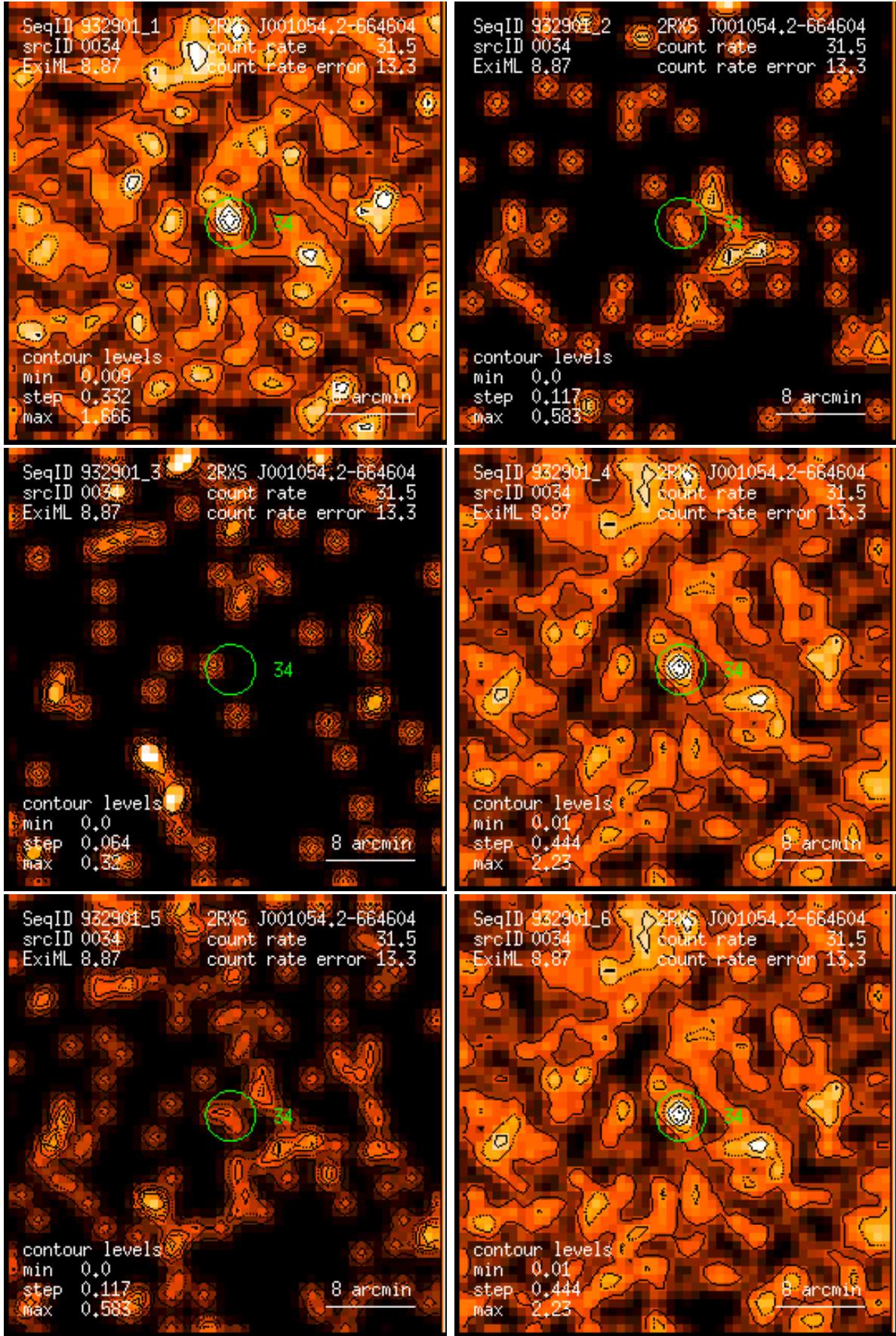
Figure 34: RASS 932901: detection 0034: band rate images, Gaussian filter: (1) PSPC channels 11 – 41, (2) 52 – 90, (3) 91 – 201, (4) 11 – 235, (5) 52 – 201, (6) 11 – 201. Broad band rates in counts/ks. Band rate contour levels in counts/ks/arcmin 2 .
