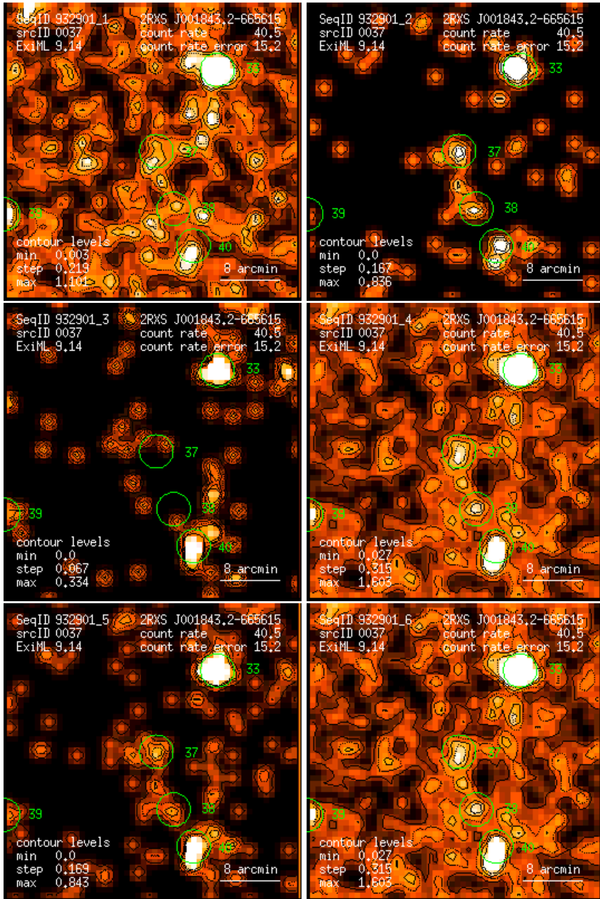
Figure 37: RASS 932901: detection 0037: band rate images, Gaussian filter: (1) PSPC channels 11 – 41, (2) 52 – 90, (3) 91 – 201, (4) 11 – 235, (5) 52 – 201, (6) 11 – 201. Broad band rates in counts/ks. Band rate contour levels in counts/ks/arcmin 2 .
