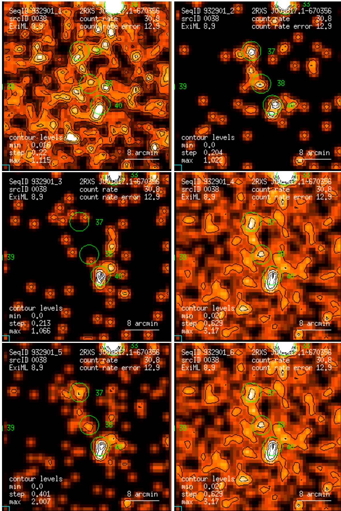
Figure 38: RASS 932901: detection 0038: band rate images, Gaussian filter: (1) PSPC channels 11 – 41, (2) 52 – 90, (3) 91 – 201, (4) 11 – 235, (5) 52 – 201, (6) 11 – 201. Broad band rates in counts/ks. Band rate contour levels in counts/ks/arcmin 2 .
