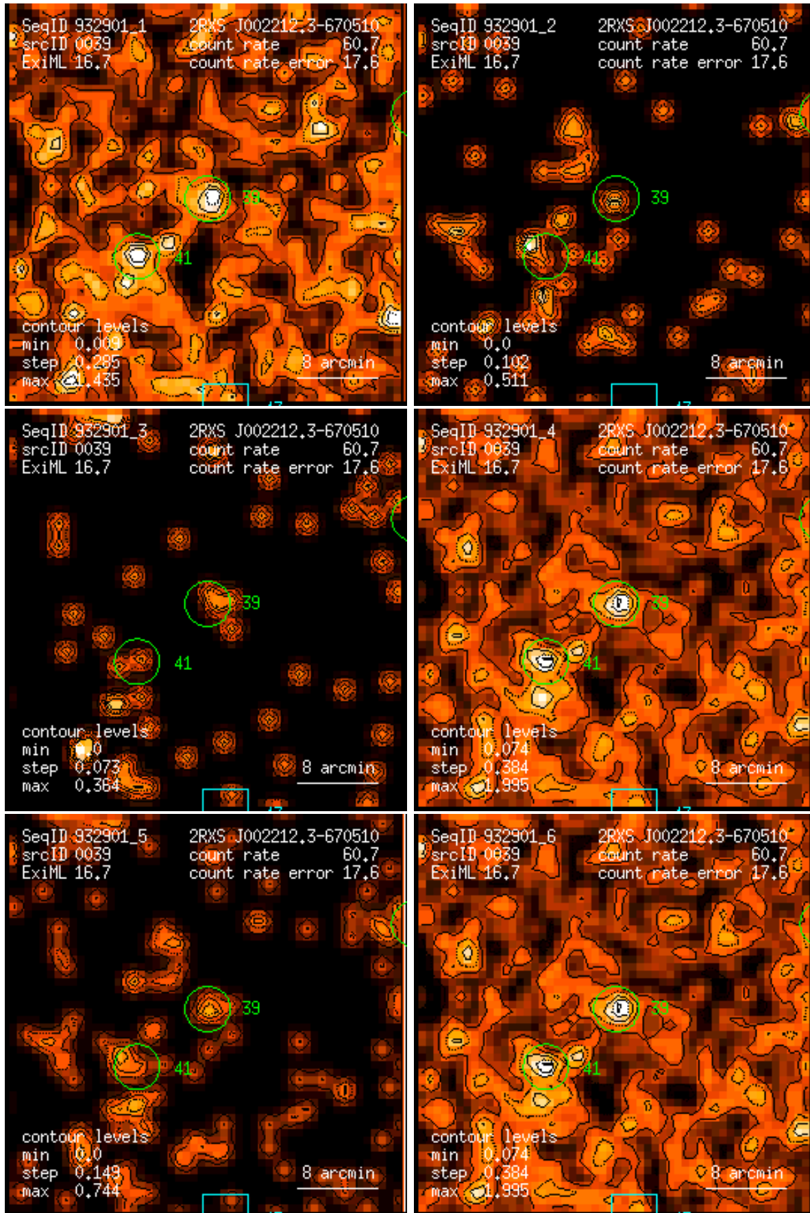
Figure 39: RASS 932901: detection 0039: band rate images, Gaussian filter: (1) PSPC channels 11 – 41, (2) 52 – 90, (3) 91 – 201, (4) 11 – 235, (5) 52 – 201, (6) 11 – 201. Broad band rates in counts/ks. Band rate contour levels in counts/ks/arcmin 2 .
