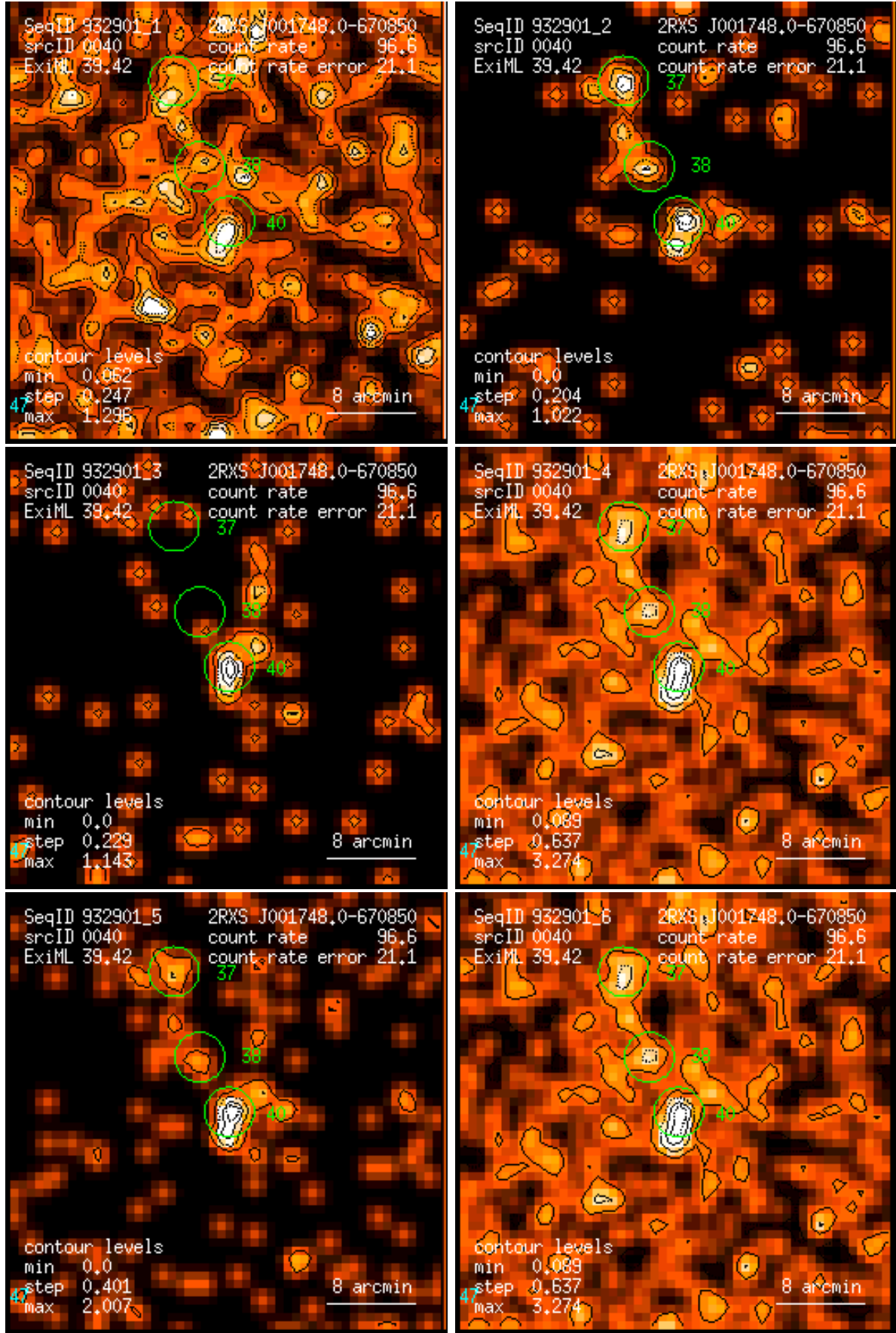
Figure 40: RASS 932901: detection 0040: band rate images, Gaussian filter: (1) PSPC channels 11 – 41, (2) 52 – 90, (3) 91 – 201, (4) 11 – 235, (5) 52 – 201, (6) 11 – 201. Broad band rates in counts/ks. Band rate contour levels in counts/ks/arcmin 2 .
