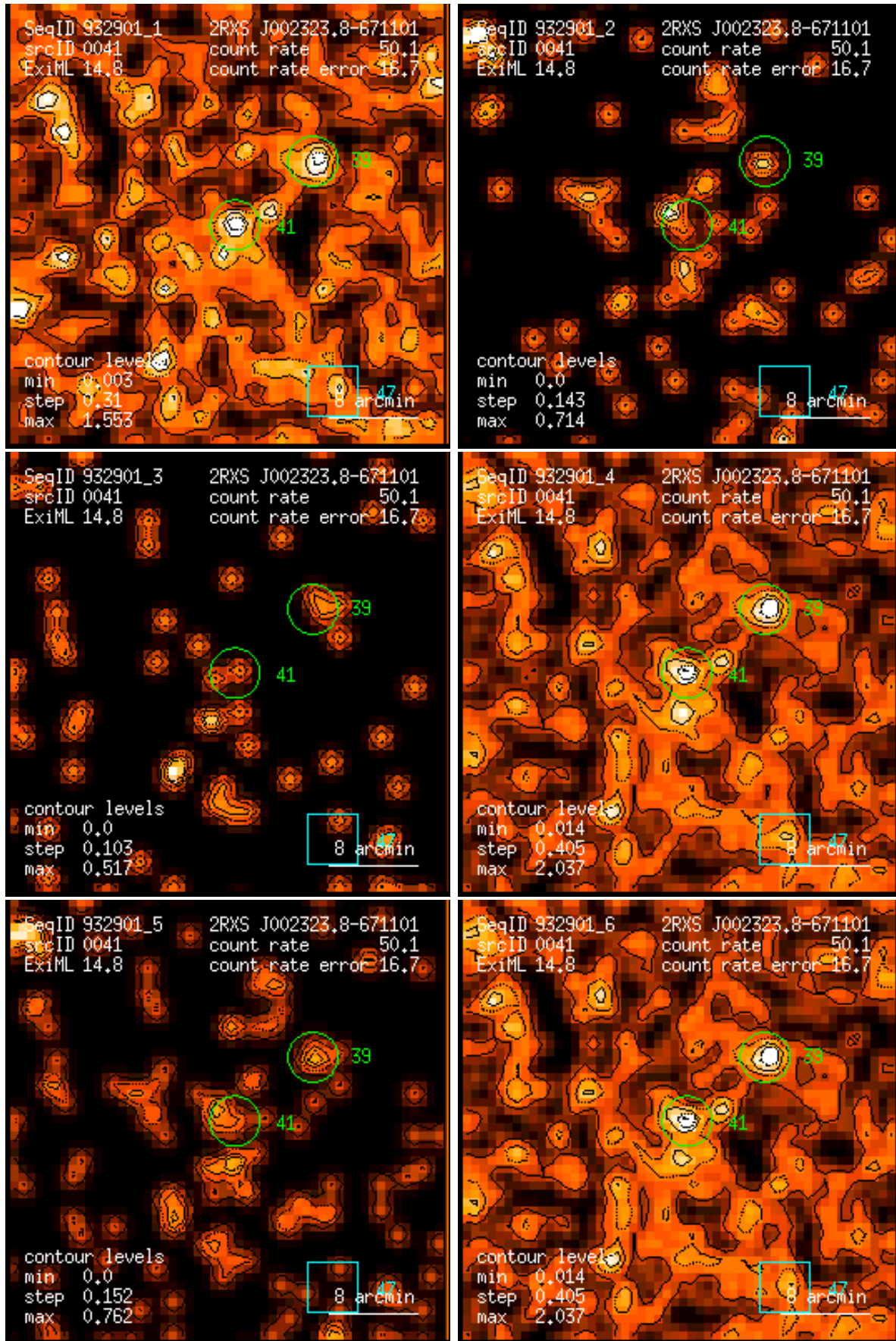
Figure 41: RASS 932901: detection 0041: band rate images, Gaussian filter: (1) PSPPC channels 11 – 41, (2) 52 – 90, (3) 91 – 201, (4) 11 – 235, (5) 52 – 201, (6) 11 – 201. Broad band rates in counts/ks. Band rate contour levels in counts/ks/arcmin 2 .
