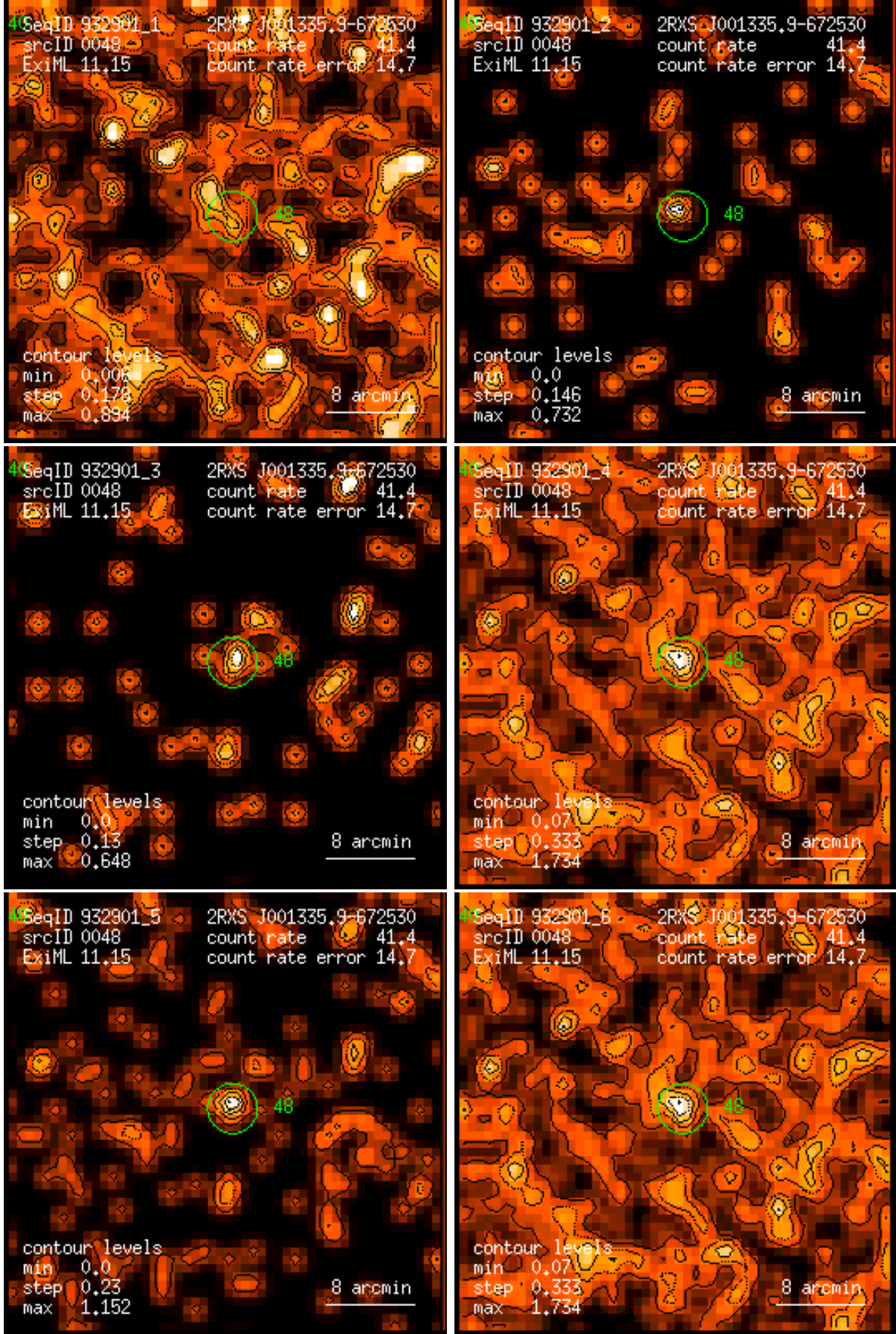
Figure 48: RASS 932901: detection 0048: band rate images, Gaussian filter: (1) PSPC channels 11 – 41, (2) 52 – 90, (3) 91 – 201, (4) 11 – 235, (5) 52 – 201, (6) 11 – 201. Broad band rates in counts/ks. Band rate contour levels in counts/ks/arcmin 2 .
