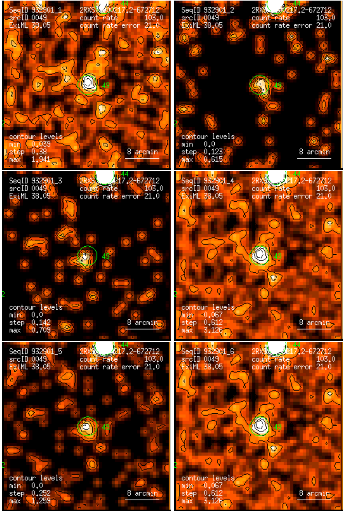
Figure 49: RASS 932901: detection 0049: band rate images, Gaussian filter: (1) PSPC channels 11 – 41, (2) 52 – 90, (3) 91 – 201, (4) 11 – 235, (5) 52 – 201, (6) 11 – 201. Broad band rates in counts/ks. Band rate contour levels in counts/ks/arcmin 2 .
