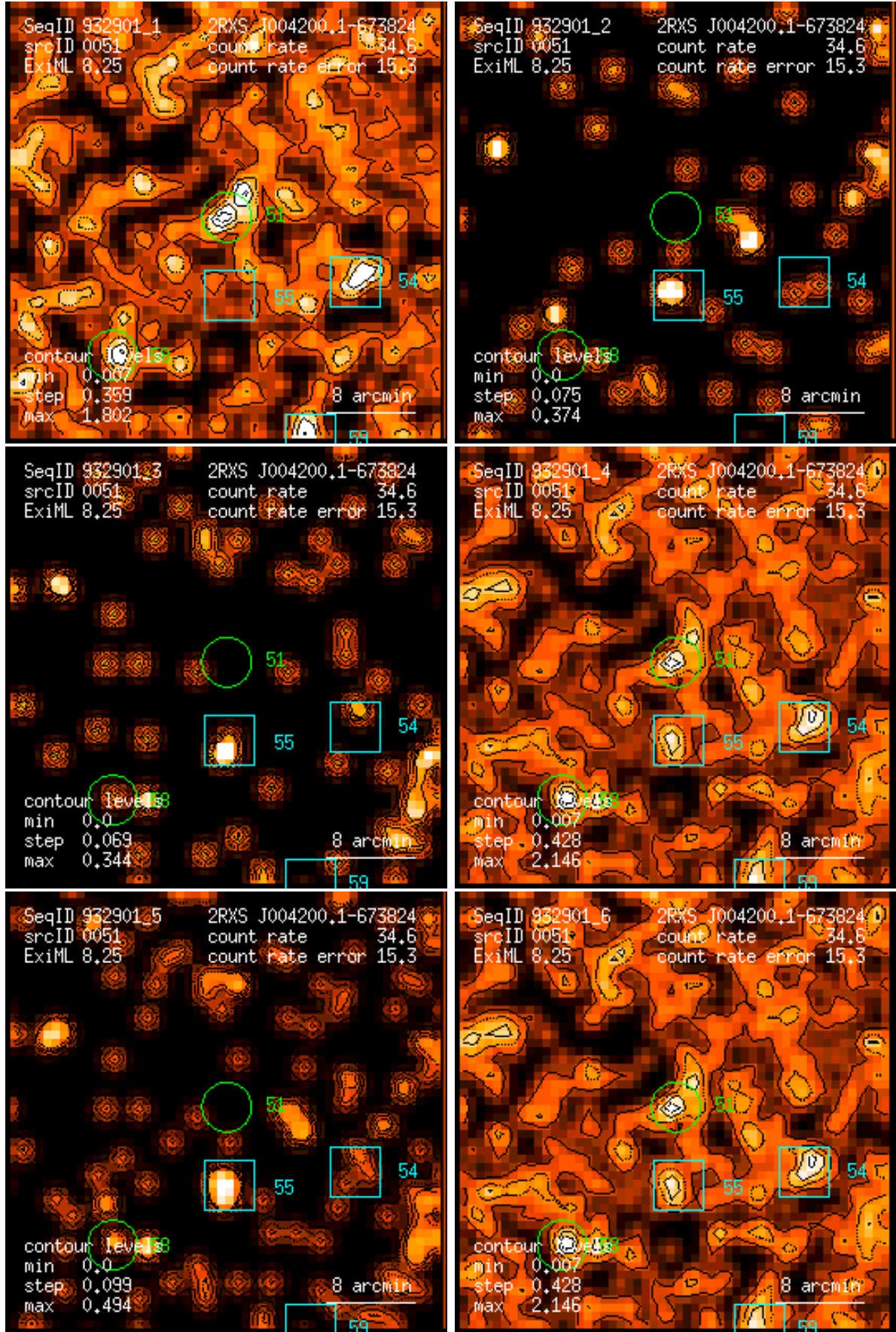
Figure 51: RASS 932901: detection 0051: band rate images, Gaussian filter: (1) PSPC channels 11 – 41, (2) 52 – 90, (3) 91 – 201, (4) 11 – 235, (5) 52 – 201, (6) 11 – 201. Broad band rates in counts/ks. Band rate contour levels in counts/ks/arcmin 2 .
