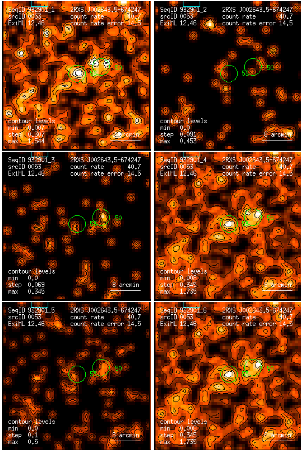
Figure 53: RASS 932901: detection 0053: band rate images, Gaussian filter: (1) PSPC channels 11 – 41, (2) 52 – 90, (3) 91 – 201, (4) 11 – 235, (5) 52 – 201, (6) 11 – 201. Broad band rates in counts/ks. Band rate contour levels in counts/ks/arcmin 2 .
