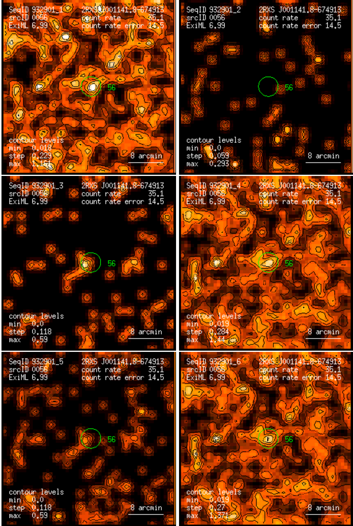
Figure 56: RASS 932901: detection 0056: band rate images, Gaussian filter: (1) PSPC channels 11 – 41, (2) 52 – 90, (3) 91 – 201, (4) 11 – 235, (5) 52 – 201, (6) 11 – 201. Broad band rates in counts/ks. Band rate contour levels in counts/ks/arcmin 2 .
