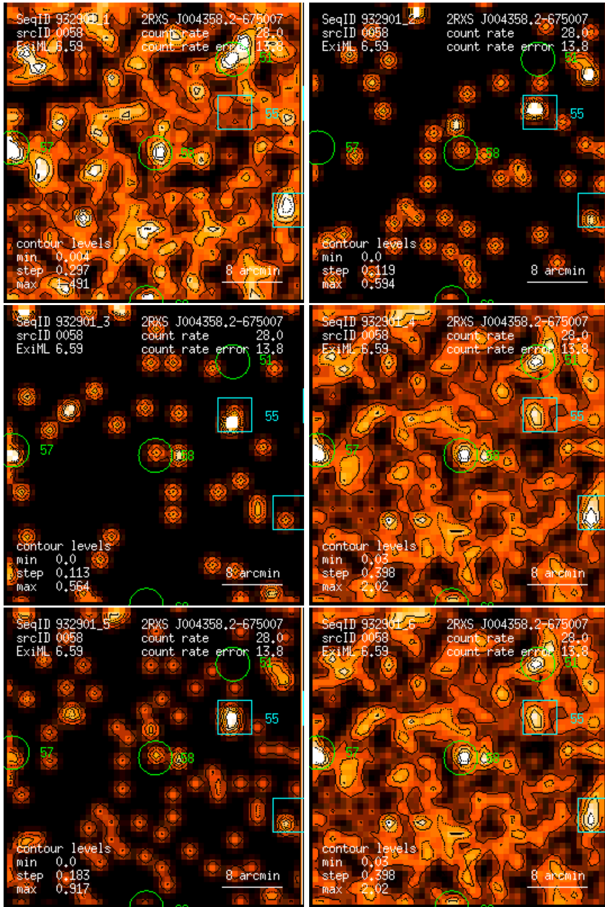
Figure 58: RASS 932901: detection 0058: band rate images, Gaussian filter: (1) PSPC channels 11 – 41, (2) 52 – 90, (3) 91 – 201, (4) 11 – 235, (5) 52 – 201, (6) 11 – 201. Broad band rates in counts/ks. Band rate contour levels in counts/ks/arcmin 2 .
