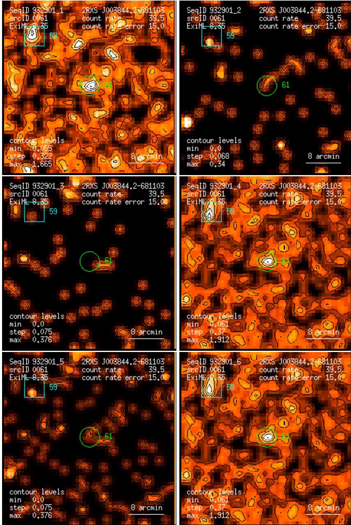
Figure 61: RASS 932901: detection 0061: band rate images, Gaussian filter: (1) PSPC channels 11 – 41, (2) 52 – 90, (3) 91 – 201, (4) 11 – 235, (5) 52 – 201, (6) 11 – 201. Broad band rates in counts/ks. Band rate contour levels in counts/ks/arcmin 2 .
