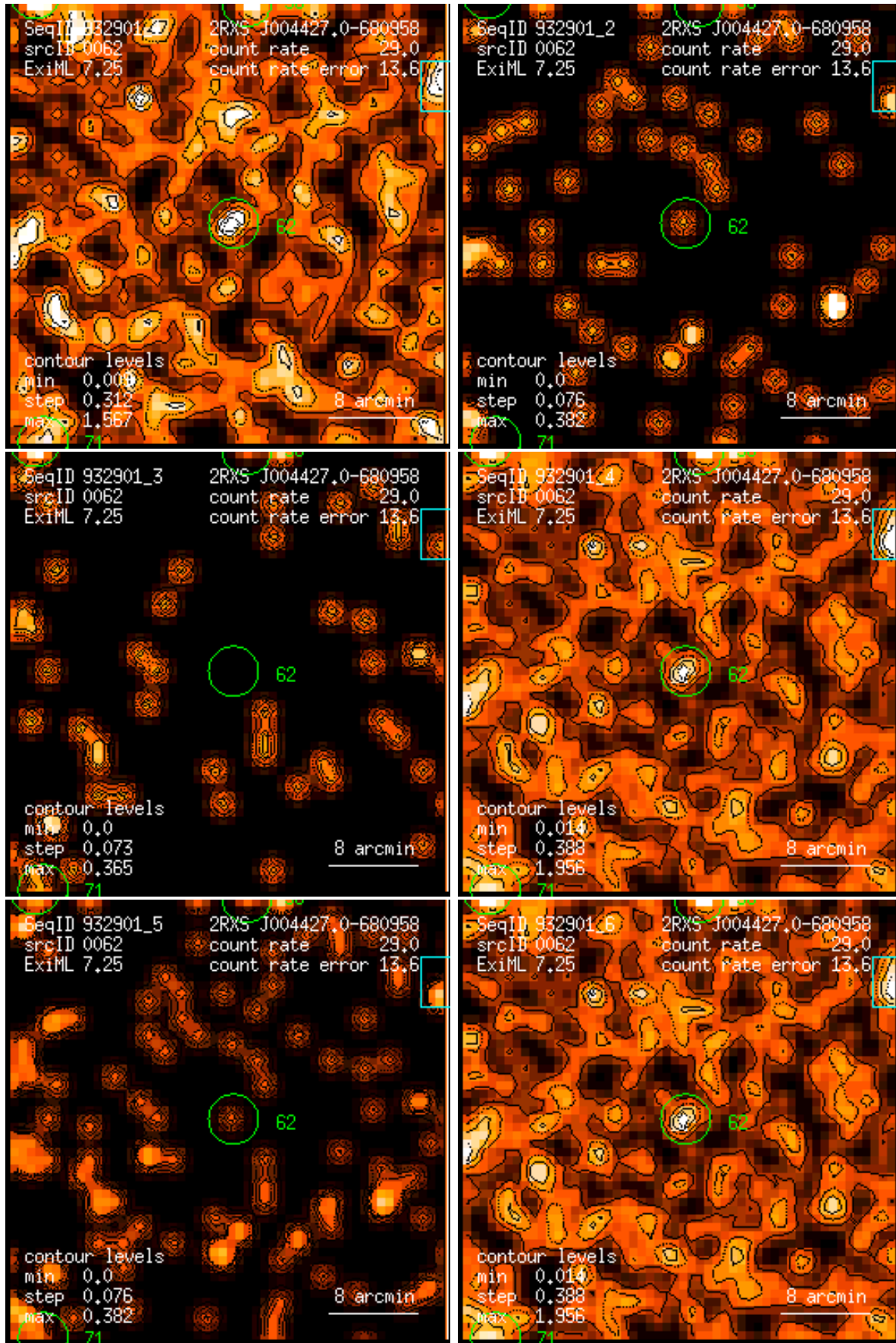
Figure 62: RASS 932901: detection 0062: band rate images, Gaussian filter: (1) PSPC channels 11 – 41, (2) 52 – 90, (3) 91 – 201, (4) 11 – 235, (5) 52 – 201, (6) 11 – 201. Broad band rates in counts/ks. Band rate contour levels in counts/ks/arcmin 2 .
