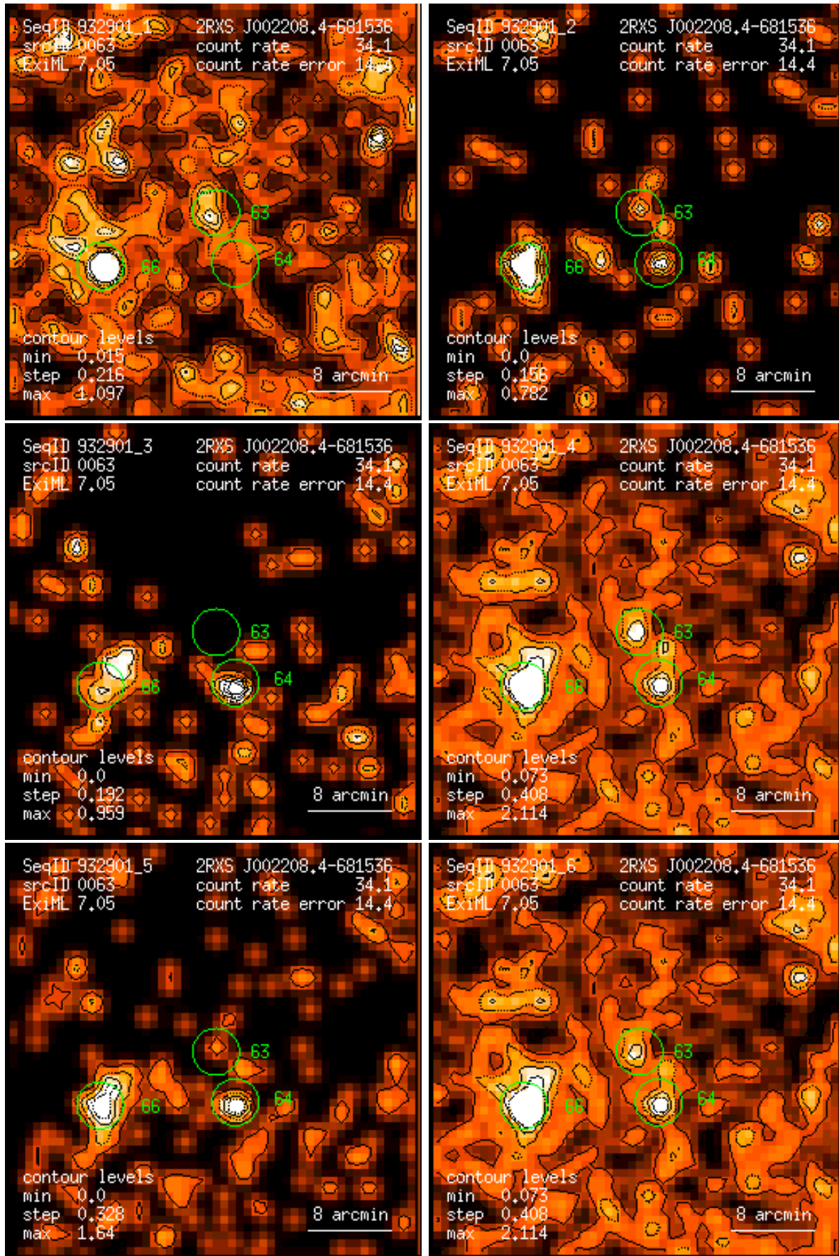
Figure 63: RASS 932901: detection 0063: band rate images, Gaussian filter: (1) PSPC channels 11 – 41, (2) 52 – 90, (3) 91 – 201, (4) 11 – 235, (5) 52 – 201, (6) 11 – 201. Broad band rates in counts/ks. Band rate contour levels in counts/ks/arcmin 2 .
