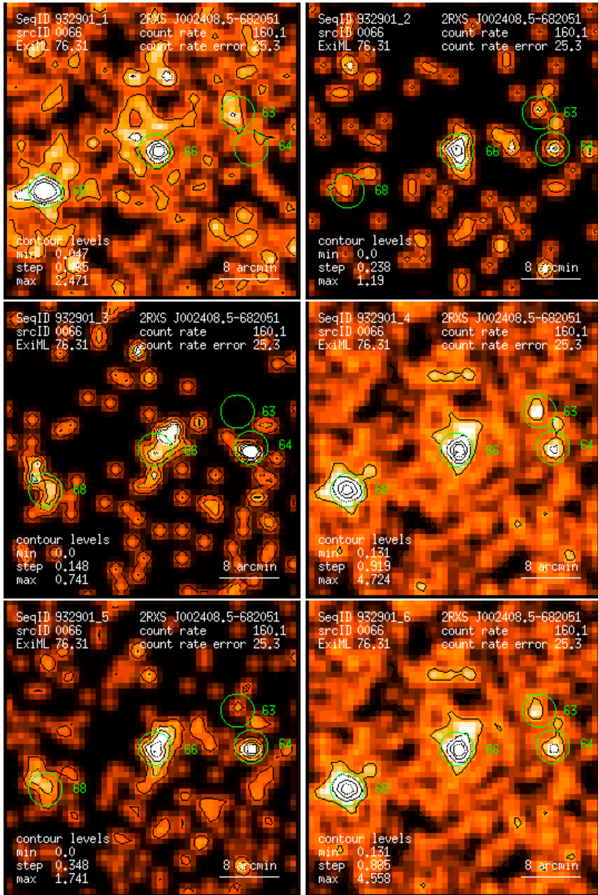
Figure 66: RASS 932901: detection 0066: band rate images, Gaussian filter: (1) PSPC channels 11 – 41, (2) 52 – 90, (3) 91 – 201, (4) 11 – 235, (5) 52 – 201, (6) 11 – 201. Broad band rates in counts/ks. Band rate contour levels in counts/ks/arcmin 2 .
