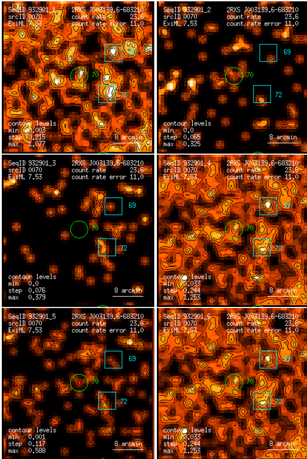
Figure 70: RASS 932901: detection 0070: band rate images, Gaussian filter: (1) PSPC channels 11 – 41, (2) 52 – 90, (3) 91 – 201, (4) 11 – 235, (5) 52 – 201, (6) 11 – 201. Broad band rates in counts/ks. Band rate contour levels in counts/ks/arcmin 2 .
