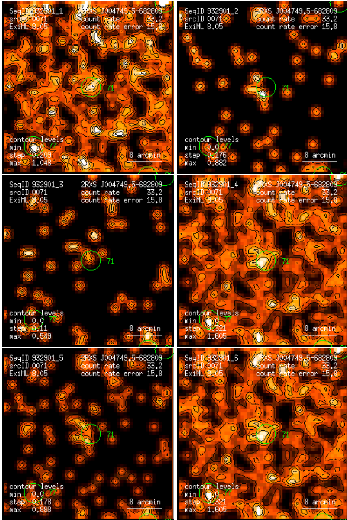
Figure 71: RASS 932901: detection 0071: band rate images, Gaussian filter: (1) PSPC channels 11 – 41, (2) 52 – 90, (3) 91 – 201, (4) 11 – 235, (5) 52 – 201, (6) 11 – 201. Broad band rates in counts/ks. Band rate contour levels in counts/ks/arcmin 2 .
