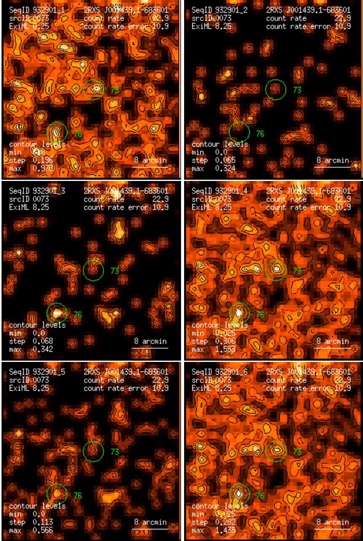
Figure 73: RASS 932901: detection 0073: band rate images, Gaussian filter: (1) PSPC channels 11 – 41, (2) 52 – 90, (3) 91 – 201, (4) 11 – 235, (5) 52 – 201, (6) 11 – 201. Broad band rates in counts/ks. Band rate contour levels in counts/ks/arcmin 2 .
