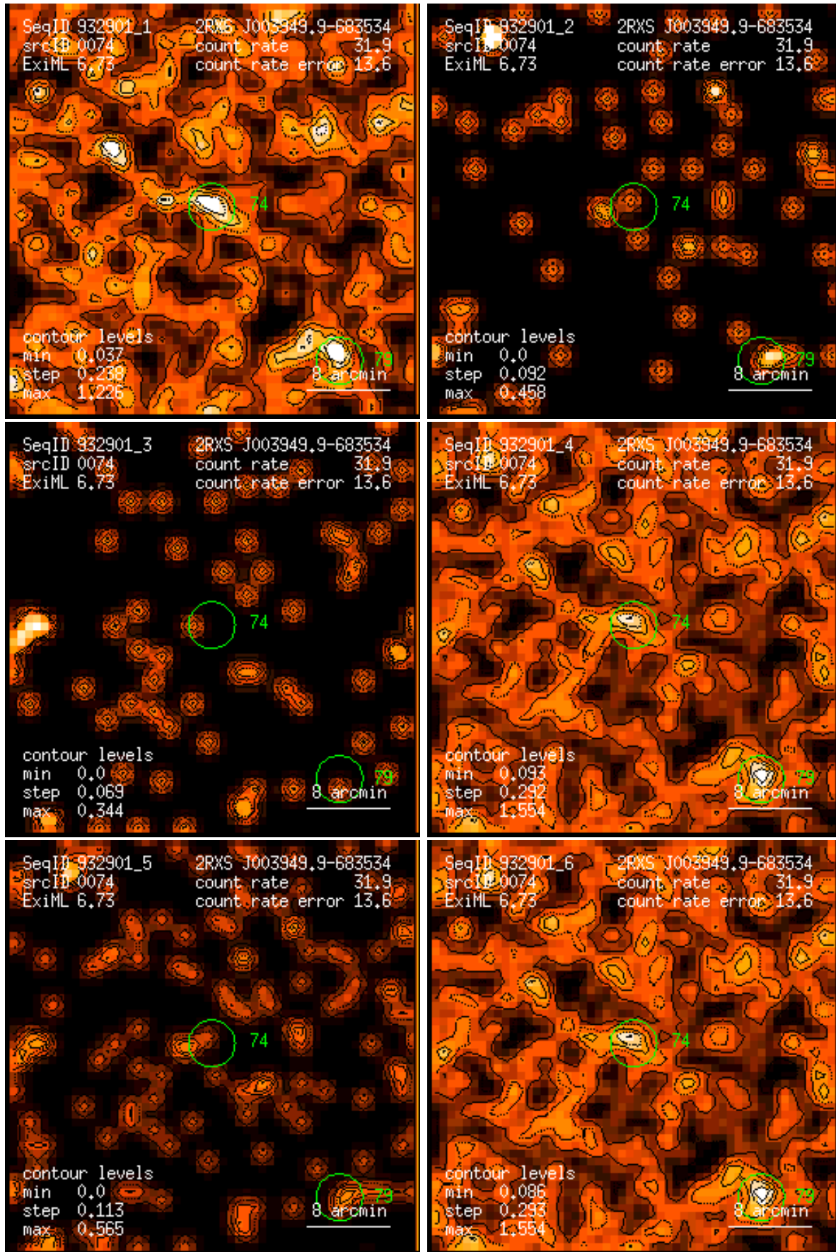
Figure 74: RASS 932901: detection 0074: band rate images, Gaussian filter: (1) PSPC channels 11 – 41, (2) 52 – 90, (3) 91 – 201, (4) 11 – 235, (5) 52 – 201, (6) 11 – 201. Broad band rates in counts/ks. Band rate contour levels in counts/ks/arcmin 2 .
