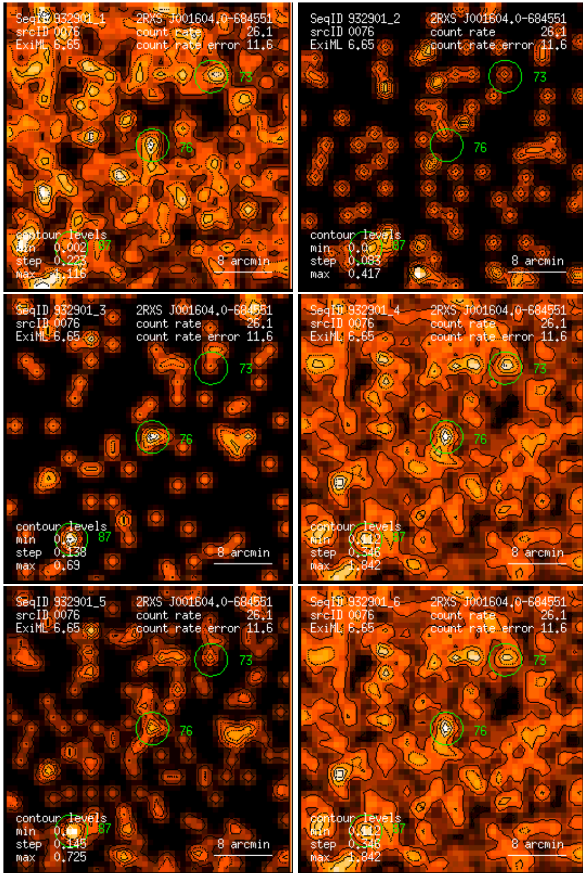
Figure 76: RASS 932901: detection 0076: band rate images, Gaussian filter: (1) PSPC channels 11 – 41, (2) 52 – 90, (3) 91 – 201, (4) 11 – 235, (5) 52 – 201, (6) 11 – 201. Broad band rates in counts/ks. Band rate contour levels in counts/ks/arcmin 2 .
