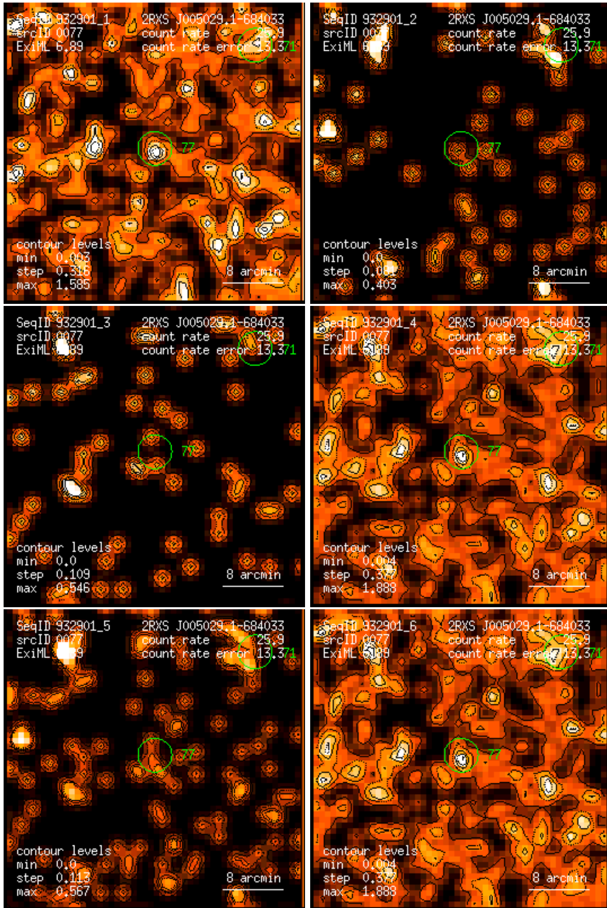
Figure 77: RASS 932901: detection 0077: band rate images, Gaussian filter: (1) PSPC channels 11 – 41, (2) 52 – 90, (3) 91 – 201, (4) 11 – 235, (5) 52 – 201, (6) 11 – 201. Broad band rates in counts/ks. Band rate contour levels in counts/ks/arcmin 2 .
