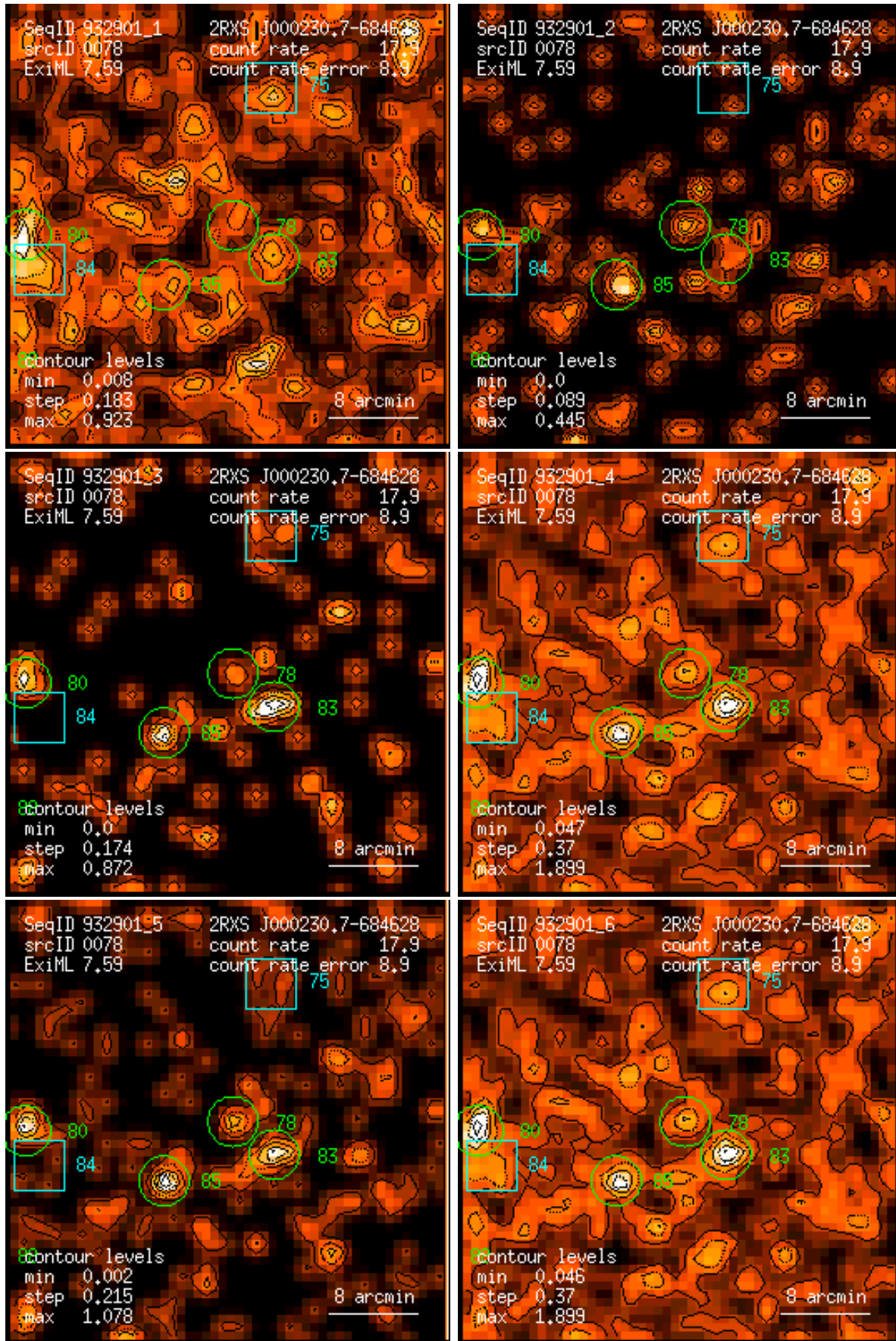
Figure 78: RASS 932901: detection 0078: band rate images, Gaussian filter: (1) PSPC channels 11 – 41, (2) 52 – 90, (3) 91 – 201, (4) 11 – 235, (5) 52 – 201, (6) 11 – 201. Broad band rates in counts/ks. Band rate contour levels in counts/ks/arcmin 2 .
