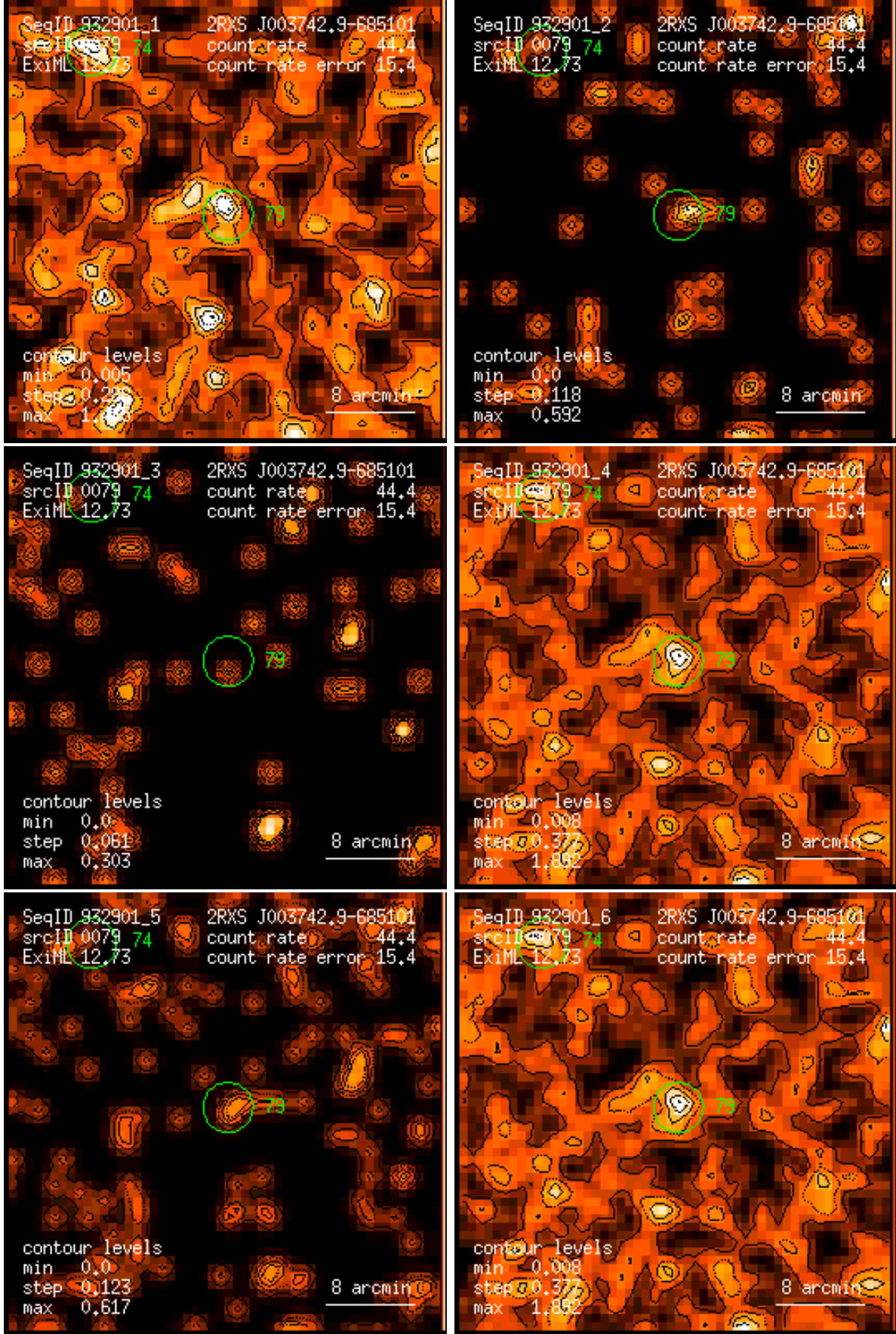
Figure 79: RASS 932901: detection 0079: band rate images, Gaussian filter: (1) PSPC channels 11 – 41, (2) 52 – 90, (3) 91 – 201, (4) 11 – 235, (5) 52 – 201, (6) 11 – 201. Broad band rates in counts/ks. Band rate contour levels in counts/ks/arcmin 2 .
