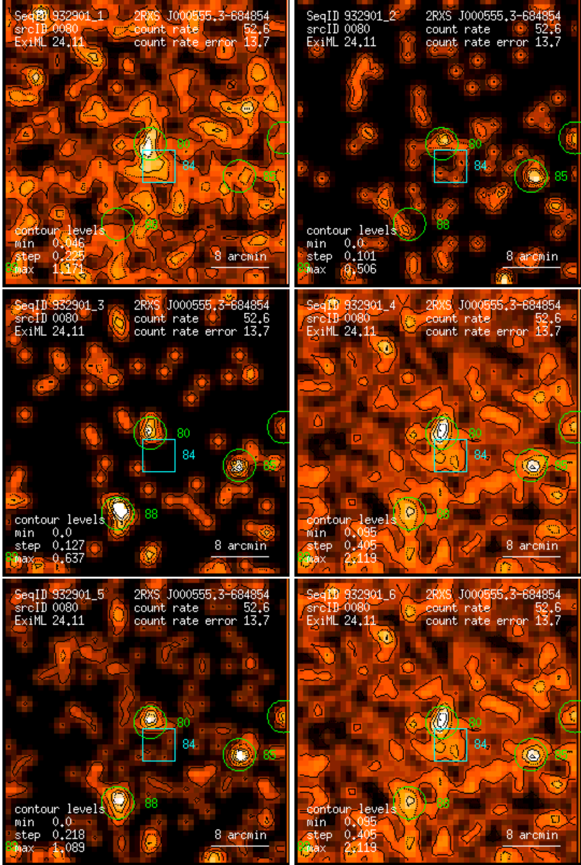
Figure 80: RASS 932901: detection 0080: band rate images, Gaussian filter: (1) PSPC channels 11 – 41, (2) 52 – 90, (3) 91 – 201, (4) 11 – 235, (5) 52 – 201, (6) 11 – 201. Broad band rates in counts/ks. Band rate contour levels in counts/ks/arcmin 2 .
