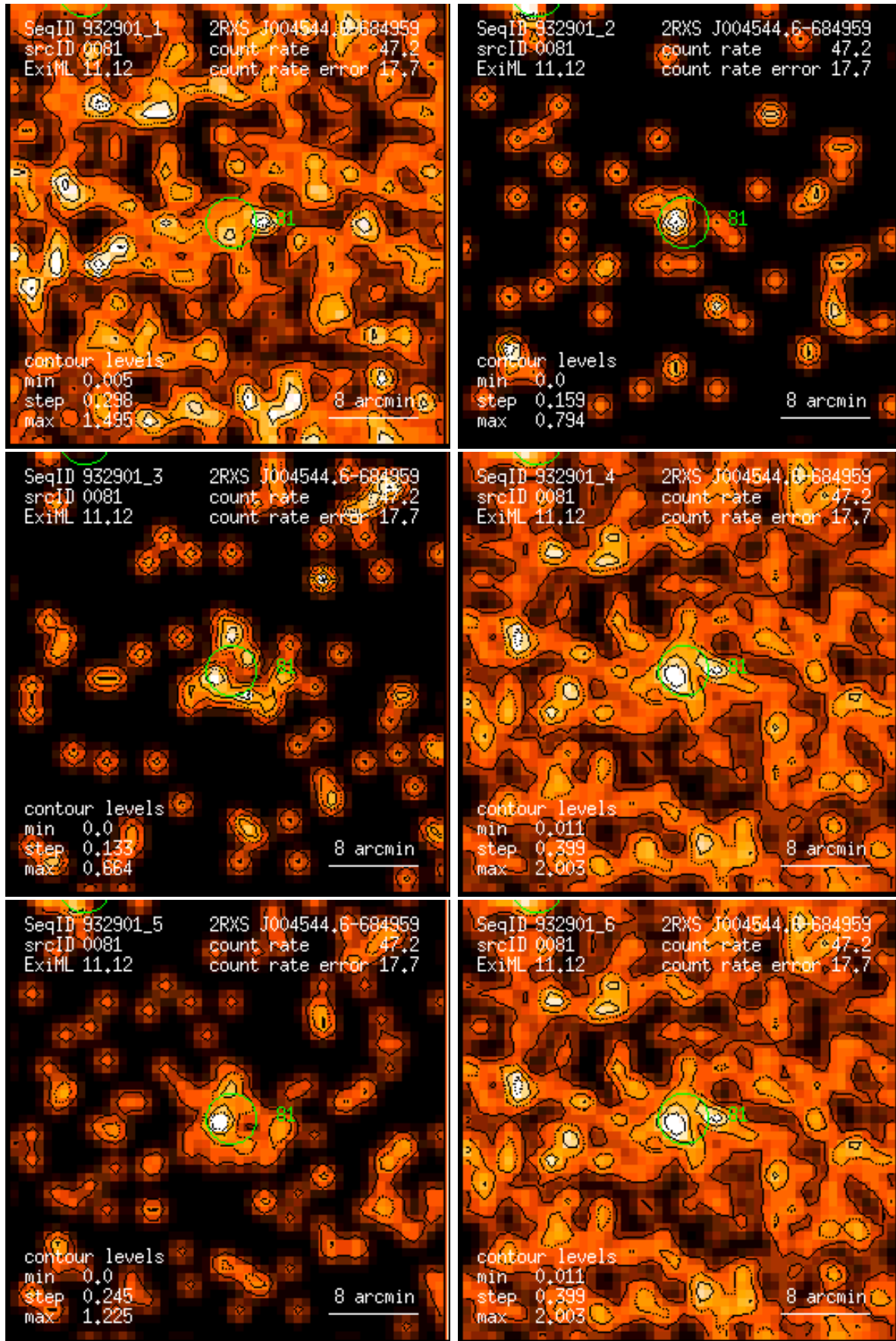
Figure 81: RASS 932901: detection 0081: band rate images, Gaussian filter: (1) PSPC channels 11 – 41, (2) 52 – 90, (3) 91 – 201, (4) 11 – 235, (5) 52 – 201, (6) 11 – 201. Broad band rates in counts/ks. Band rate contour levels in counts/ks/arcmin 2 .
